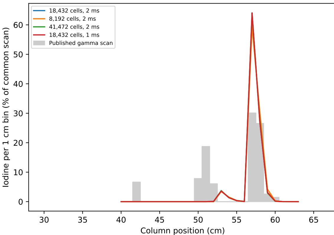
LBE, steel, 1% source saturation
