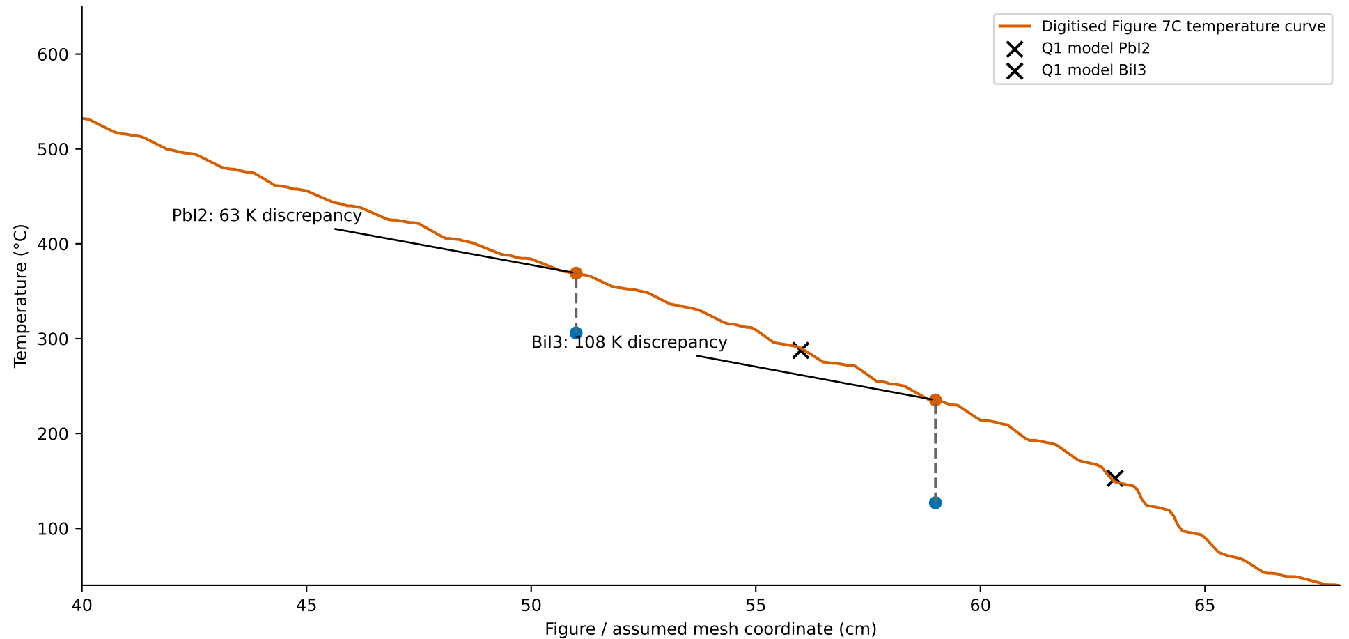
Silica: curve and printed temperatures do not agree at measured scan peaks
