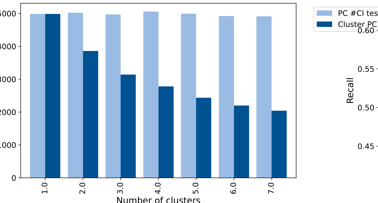
Number of CI tests needed for different numbers of clusters
