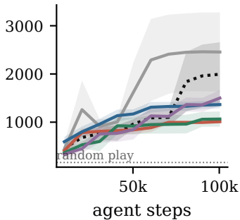
Q*bert
