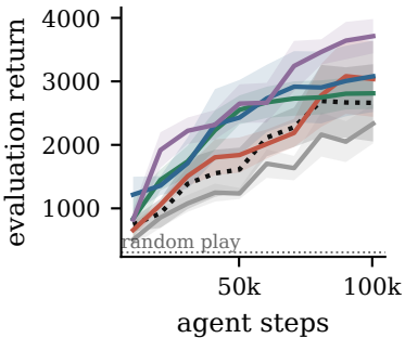
Ms. Pac-Man
