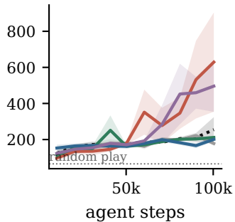
Frostbite
