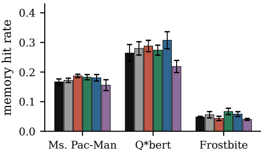
Neighbor retrieval (MFEC)
