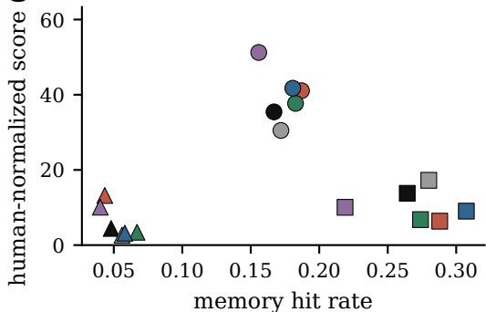
Retrieval vs. performance (MFEC)
