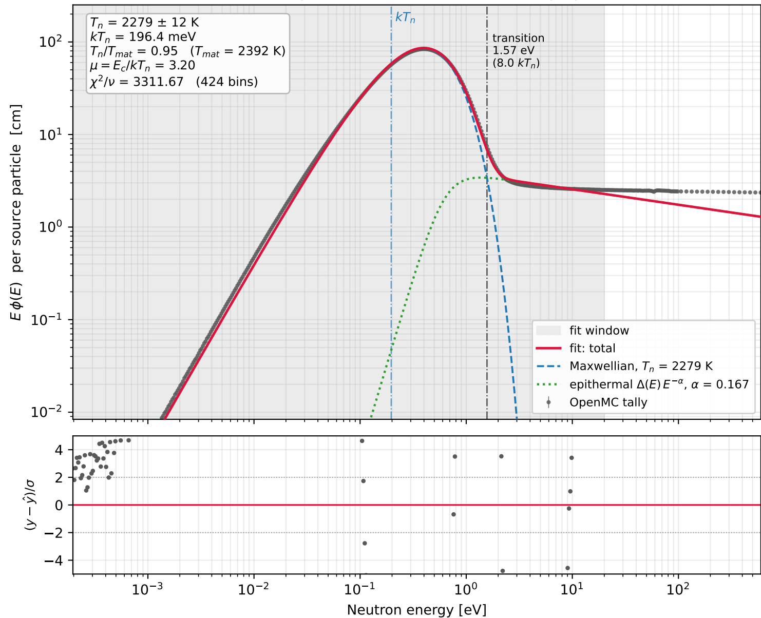
Thermal spectrum and Maxwellian fit -- graphite
