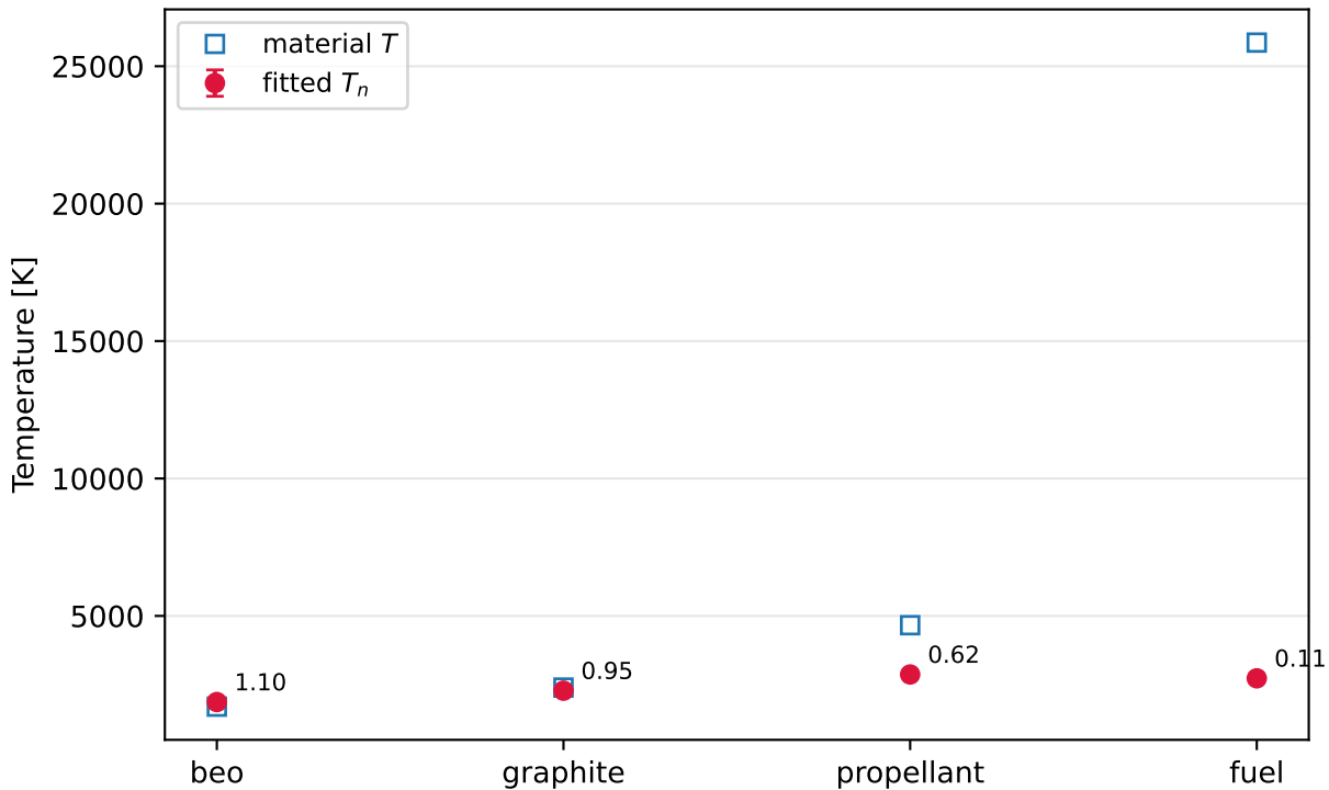
Neutron temperature vs material temperature
