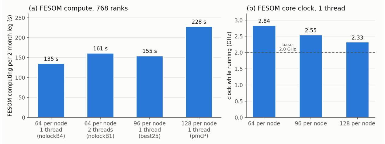
Figure 2: (a) FESOM computing time per 2-month leg (LUCIA timelines) for the same 768 ranks and binary in four layouts. The second OpenMP thread costs 19 % against leaving its core idle; packing 128 ranks per node costs 69 %. (b) Clock of the busy FESOM cores while they run, from hardware counters: the fewer cores of a node are busy, the higher the rest boost above the 2.0 GHz base clock. DRAM traffic stays at 40 to 70 GB/s per node in every layout, far below what a node delivers, so the idle cores buy clock and some cache, not bandwidth.
