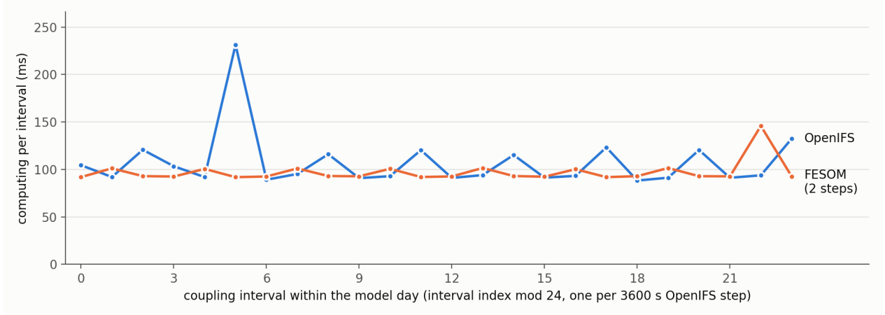
Figure 3: Computing time per coupling interval in TEST_best25, averaged over the 59 model days by position in the day. In ordinary intervals FESOM (two steps, 92–102 ms) is now as long as OpenIFS (88–95 ms); the long intervals are OpenIFS’s radiation steps (every third, 115–133 ms), one OpenIFS output interval (231 ms) and one FESOM output interval (146 ms) per day. FESOM is the longer component in 823 of 1414 intervals. The critical path is 163.7 s; OpenIFS 20 % faster alone would shorten it by 8.5 %, an infinitely fast FESOM by 7 %.
