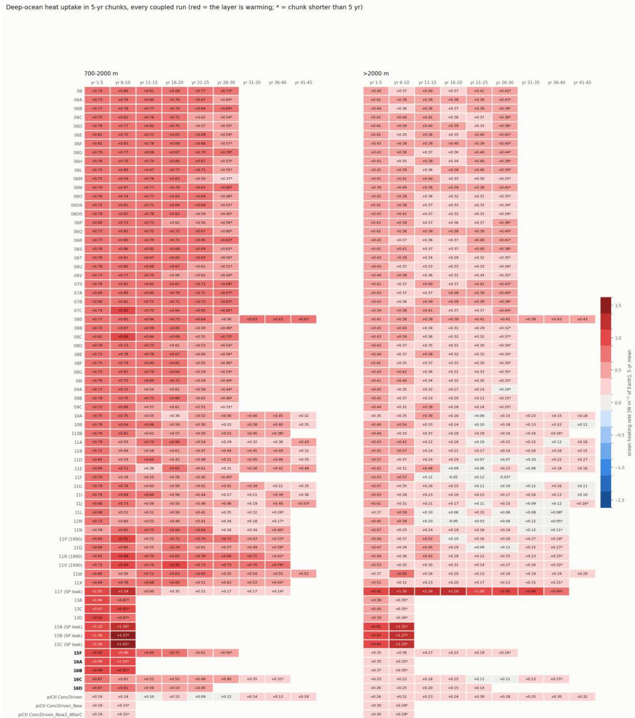
Figure 43: Ocean heating rate in 5-year chunks at 700–2000 m (left) and below 2000 m (right), in \text{W m}^{-2} of Earth area so it compares directly with TOA. From annual-mean temperature, \rho c_p T A \Delta z with below-bottom points masked, on each run’s own mesh. * marks a chunk shorter than 5 years. Every run starts at 0.7–1.0 at mid-depth; only the new-sea-ice chain lets it decay.
