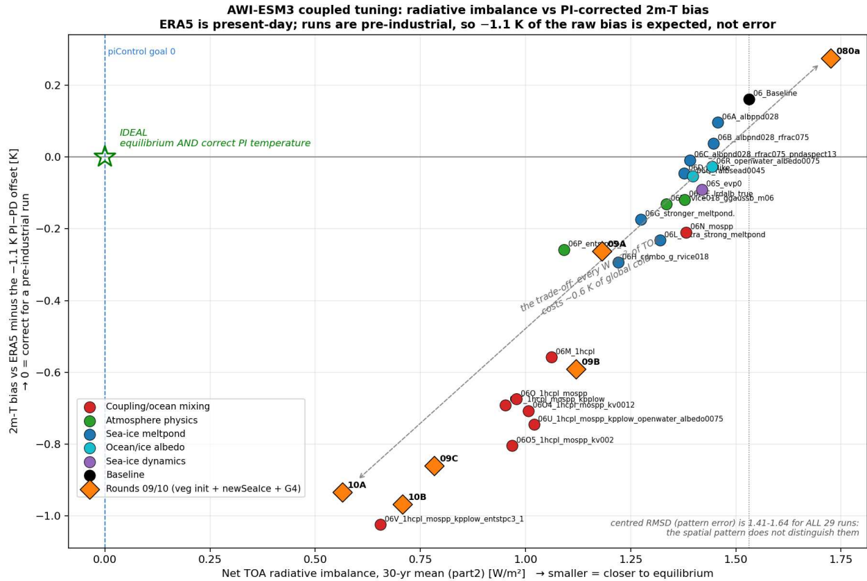
Figure 4: Net TOA imbalance against 2 m-T bias vs ERA5, corrected for the reference period (ERA5 is present-day, the runs pre-industrial, \approx 1.1\text{ K} apart, so 0 is correct for a PI run). The runs lie on a line, not in a cloud: from 080a at (1.73, +0.28) to 10A at (0.57, -0.93 ), every \text{W m}^{-2} of TOA improvement has cost \approx 0.6\text{ K} of global cold. And the spatial pattern is not what distinguishes them — centred RMSD, \sqrt{\text{RMSD}^2 - \text{bias}^2} , is 1.41–1.64 K across all 29 runs, a \pm 8\% spread against a raw-RMSD spread of 64 %. The entire apparent skill difference between these runs is one number: the global mean.
