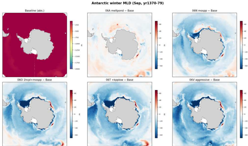
Figure 2: Antarctic September mixed-layer depth: Baseline absolute (top-left, own scale), others anomaly vs Baseline on \pm 70 m. The mixing runs (06N/O/T/V) restructure Weddell/Ross winter convection; melt-pond (06A) barely touches it. The mechanism is real and the direction is right — the objection in §3 is to how much of the radiative target is being bought this way, not to the ocean physics.
