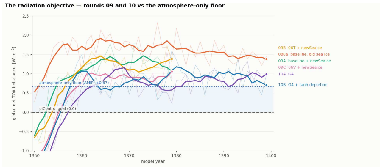
Figure 1: Global-mean net TOA by model year; thin annual, bold 5-yr running mean. G4 is worth \approx 0.25 \text{ W m}^{-2} at top of atmosphere — 10A settles at +0.854 against 09C’s \approx 1.06 , the best of the previous round. The dotted line is the atmosphere-only floor of +0.67 measured directly by AMIP; the shaded band is the only part of the remaining gap that ocean-side tuning can still close, and everything above the dotted line is atmospheric. 10A and 10B are indistinguishable ( +0.854 vs +0.899 ) although 10B carries the snow scheme that destroyed the winter soil by 20 K — distributional surface damage is invisible to box-mean energy diagnostics, so TOA cannot be used as a safety check on a surface parameterisation.
