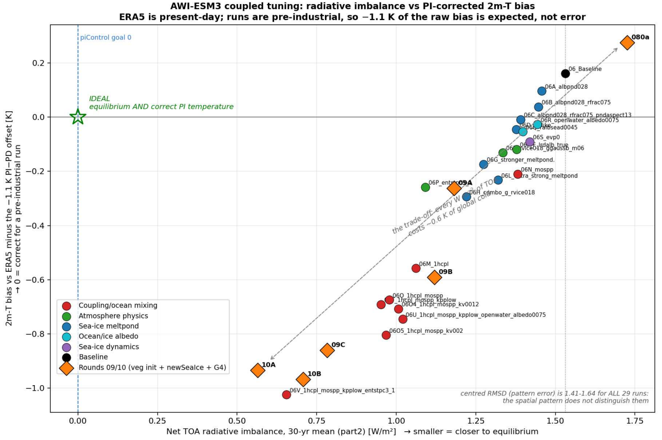
Figure 2: Net TOA imbalance (30-yr mean, part2 ) against the 2 m-T bias vs ERA5 corrected for the reference period , now including rounds 09 and 10 (orange diamonds, common window 1354–1379). ERA5 is present-day and the runs are pre-industrial, about 1.1 K apart, so that much of the raw cold bias is expected rather than error ; the y axis subtracts it, and 0 is correct for a PI run. Ranking by raw RMSD penalises exactly the runs that are correctly cold, which is why the earlier version of this figure was misleading. Dashed blue = the corrected piControl goal of 0 (§37); the star marks the ideal, which nothing occupies. The runs lie on a line, not in a cloud: every \text{W m}^{-2} of TOA improvement costs \approx 0.6 K of global cold, from 080a at (1.73, +0.28) to 10A at (0.57, -0.93 ). And the pattern error is not what distinguishes them — centred RMSD, \sqrt{\text{RMSD}^2 - \text{bias}^2} , which removes any uniform offset, is 1.41–1.64 K across all 29 runs, a \pm 8\% spread against a raw-RMSD spread of 64%. Colour = parameter family.
