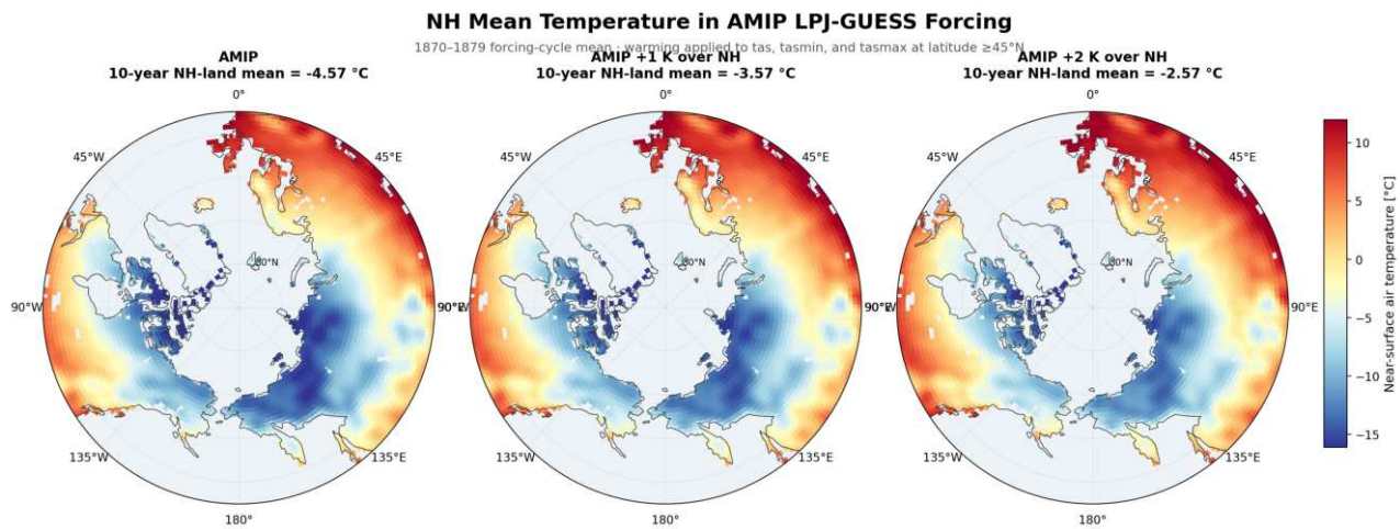
Figure 60: Input check for the planned AMIP temperature sensitivity. Ten-year NH-land mean near-surface temperature in the original, +1 K and +2 K forcing cycles. The increments were applied consistently to tas , tasmin and tasmax at latitude \geq 45^\circ\text{N} ; no vegetation response is shown because these two spin-ups have not yet been run.
