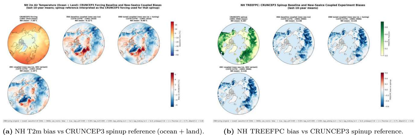
Figure 1: New-sea-ice branch update: common last-10-year means (1370–1379) for 09A/09B/09C.
