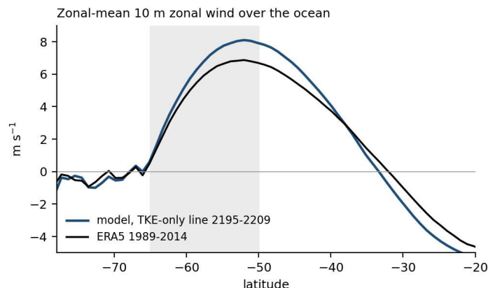
Figure 59: Zonal-mean 10 m zonal wind over the ocean. The jet is at the observed latitude (52 S) and 18 % too fast; over 50–65 S (shaded) the mean is 6.15 against 5.29 m s -1 in every season. The stress is only 10 % above ERA5 (see text). ERA5 is present day; the pre-industrial jet was weaker.
