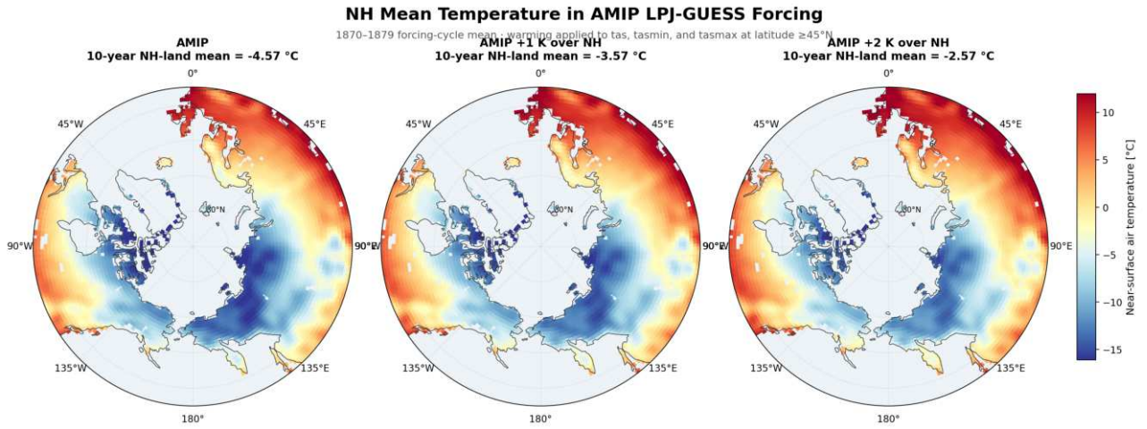
Figure 60: Input check for the planned AMIP temperature sensitivity. Ten-year NH-land mean near-surface temperature in the original, +1 K and +2 K forcing cycles. The increments were applied consistently to tas , tasmin and tasmax at latitude \geq 45^\circ\text{N} ; no vegetation response is shown because these two spin-ups have not yet been run.
