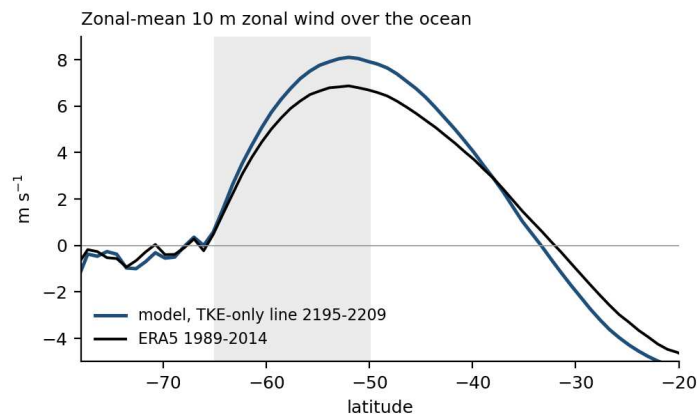
Figure 59: Zonal-mean 10 m zonal wind over the ocean. The jet is at the observed latitude (52 S) and 18 % too fast; over 50–65 S (shaded) the mean is 6.15 against 5.29 m s -1 , +35 % in u^2 , in every season. ERA5 is present day; the pre-industrial jet was weaker.
