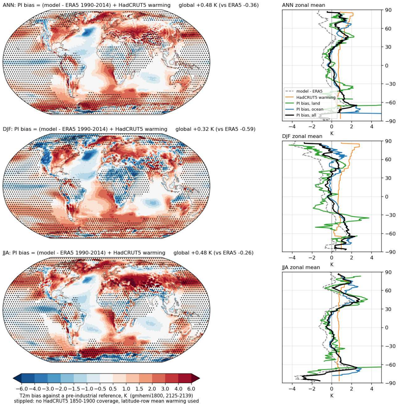
Figure 52: T2m bias of gmhemi1800 2125–2139 against a PI reference, (model – ERA5 1990–2014) + HadCRUT5 warming 1850–1900 → 1990–2014. Stippled: no HadCRUT5 1850–1900 coverage, latitude-row mean warming used. Right: zonal means for land, ocean and all, with the uncorrected model – ERA5 dashed and the HadCRUT5 warming in orange.
