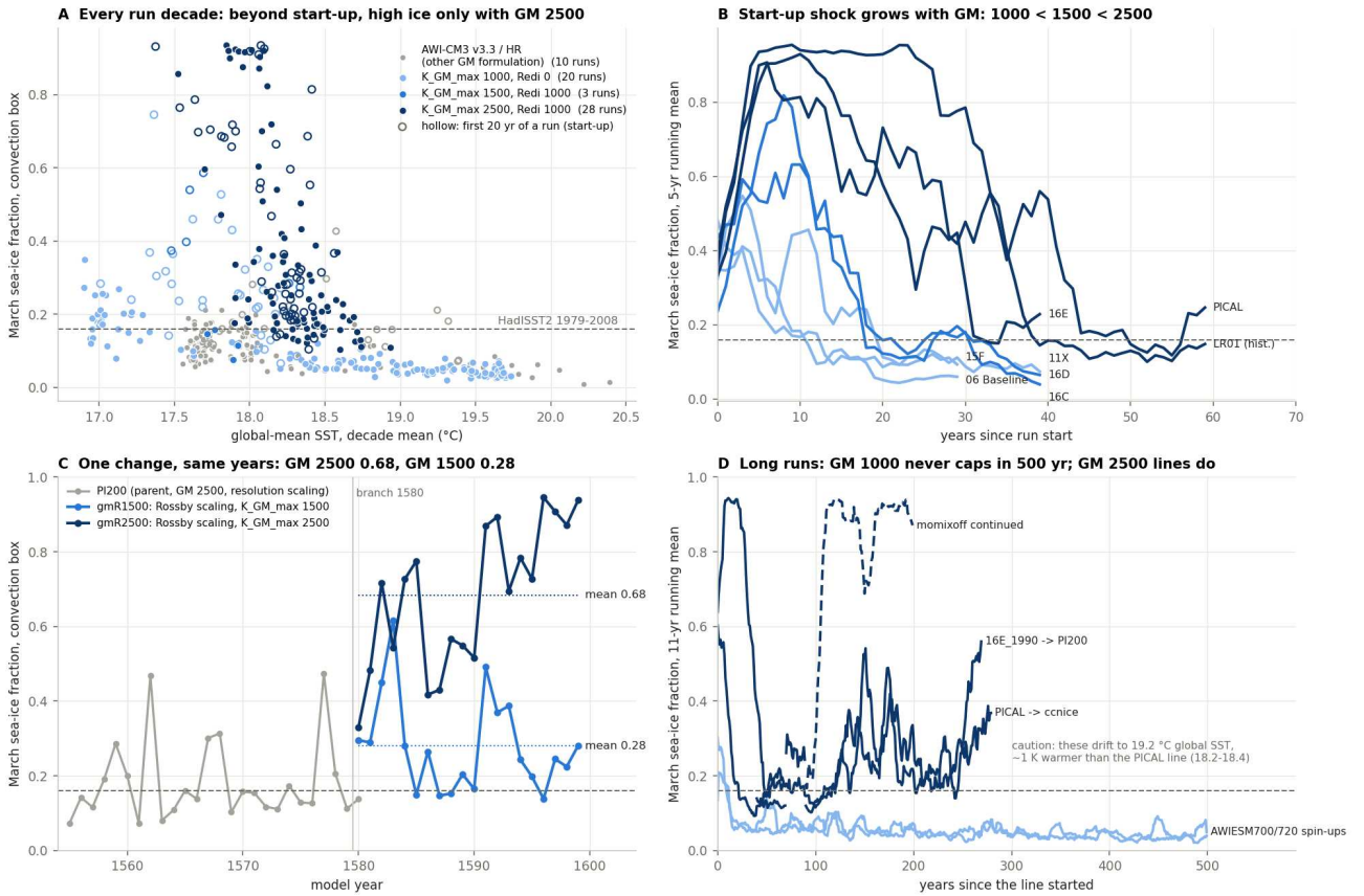
Figure 47: Labrador March ice across the run history, by GM/Redi setting. (A) every run-decade against global SST: beyond start-up, high ice only with GM 2500. (B) the start-up shock grows 1000 < 1500 < 2500. (C) one change on identical years: gmR2500 0.68 against gmR1500 0.28. (D) long runs: GM 1000 never caps in 500 years; the GM 2500 lines do.
