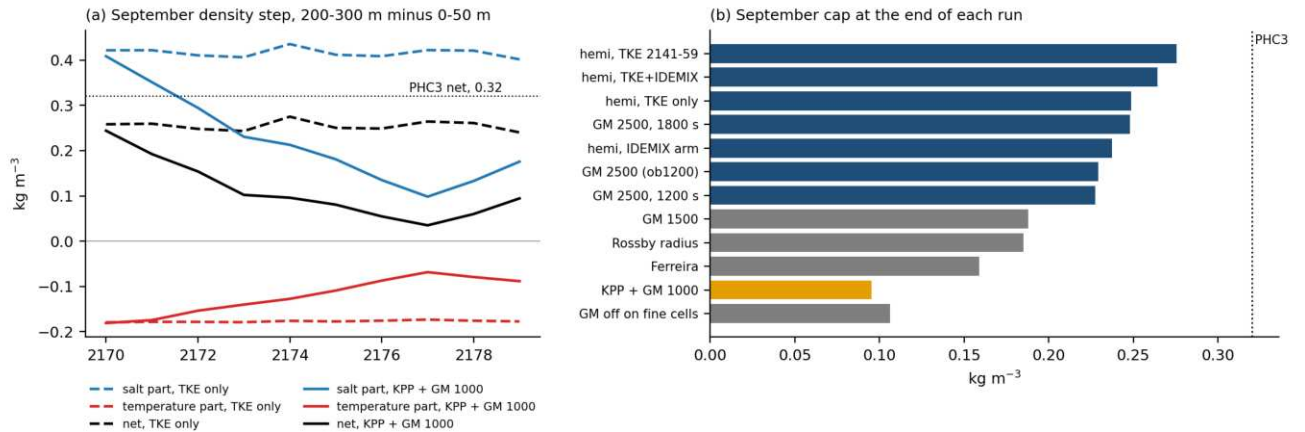
Figure 58: (a) September density step between 0–50 m and 200–300 m in the newly convecting region, split into its salt and temperature parts. In the arm the salt part collapses from 0.42 to 0.10 in seven years. (b) The same step at the end of every run with 3D output: it orders by the effective GM south of 55 S, and no run reaches the PHC3 value.
