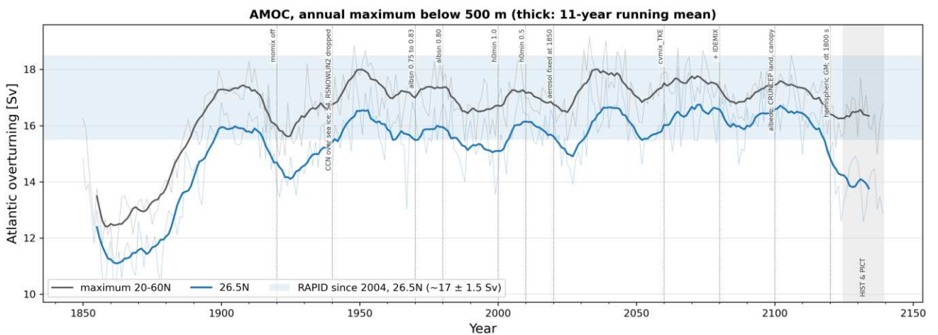
Figure 55: Atlantic overturning along the critical path: annual maximum below 500 m at 26.5 N and over 20–60 N. It spins up over the first 50 years, holds 15–16.5 Sv at 26.5 N for two centuries through every atmospheric and sea-ice change, and drops at the 2120 branch.
