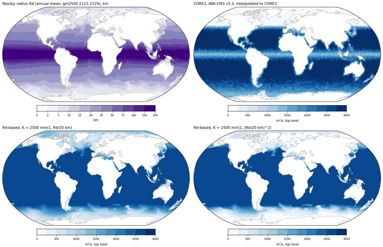
Figure 50: Rossby radius from gm2500, 2121–2129 (top left); CORE2/AWI-CM3 v3.3 GM interpolated to CORE3 (top right); two R_d -based K forms with a 20 km reference, linear (bottom left) and quadratic (bottom right).
