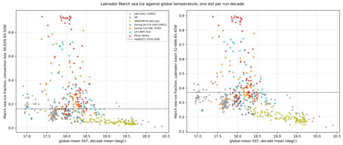
Figure 48: Labrador March ice against decade-mean global SST, one dot per run-decade, coloured by model family; convection box (left) and basin (right). The PICAL family is the cluster near 0.9 at 17.8–18.1 °C.
