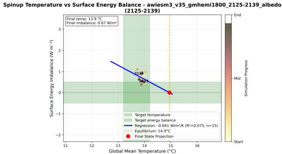
Figure 51: Corrected Gregory plot, gmhemi1800 2125–2139: global T2m against surface energy imbalance, final 0.67 \text{ W m}^{-2} . The regression explains almost nothing ( R^2 = 0.075 , n = 15 ), so its extrapolated equilibrium of 14.9^\circ\text{C} carries no weight.
