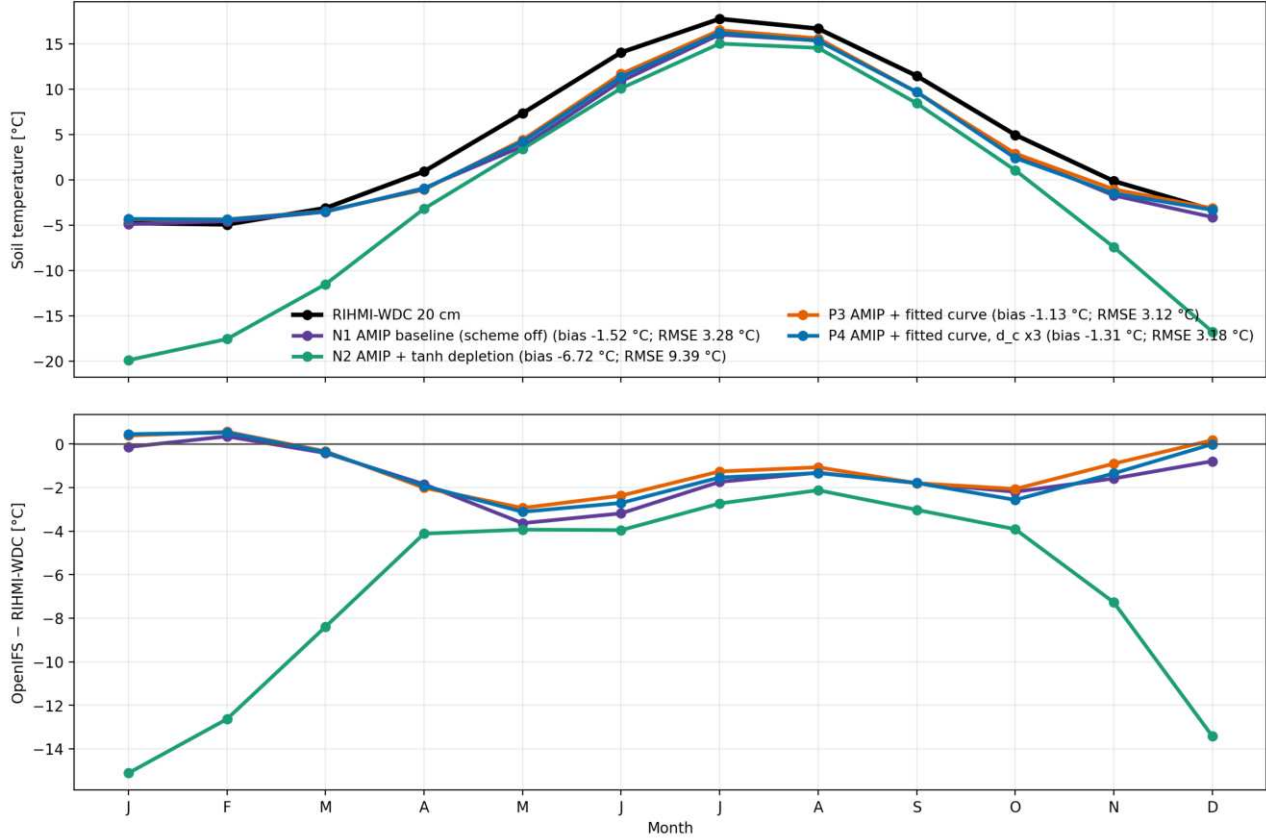
Figure 3: AMIP soil temperature against 105 RIHMI-WDC stations (st12 7–28 cm vs observed 20 cm, QC=0). The falsified tanh run (green) peels away from October and reaches -15^{\circ}\text{C} in January. The adopted runs lie on the scheme-off baseline all winter and slightly above it, and beat it on every metric — bias -1.13 vs -1.52 , RMSE 3.12 vs 3.28 . The remaining message of this figure is the April–September gap: every run including scheme-off tracks the observations through Dec–Mar and then falls 2\text{--}3.5^{\circ}\text{C} short all growing season, identically. No snow scheme can touch that — it is the global tropospheric cold bias of §6.
