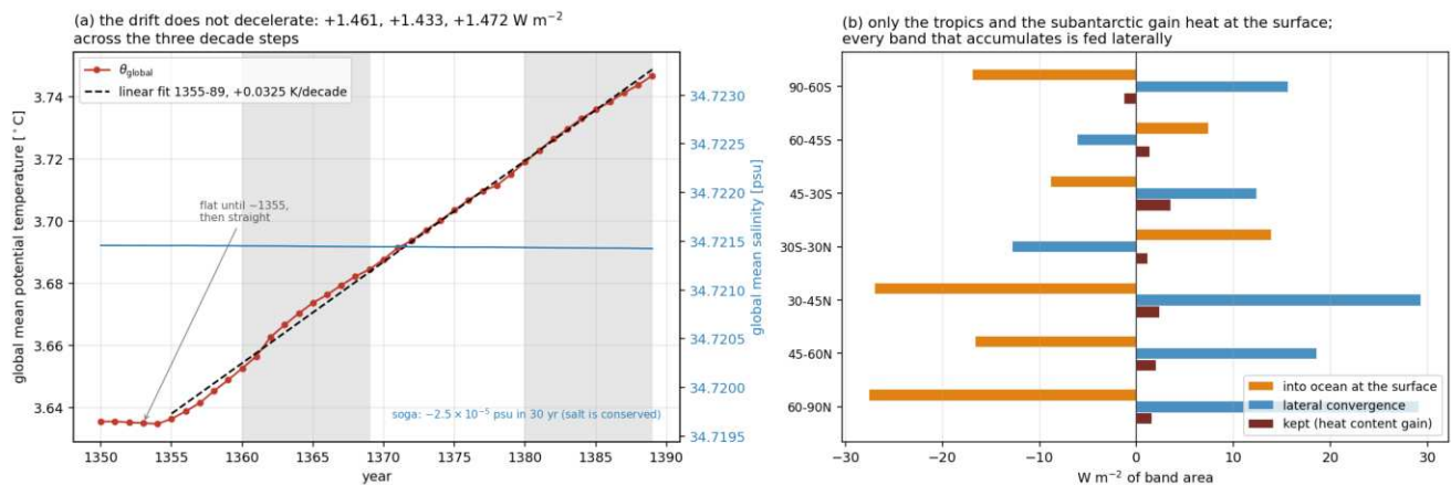
Figure 41: (a) The drift is flat for about five years after the branch and then perfectly straight: the three decade-to-decade steps are +1.461 , +1.433 and +1.472 W m^{-2} , so this is a standing bias and not an equilibrating transient. Global mean salinity (blue, right axis) drifts -2.5 \times 10^{-5} psu in 30 years — salt is conserved, which kills the virtual-salt-flux hypothesis. (b) Only the tropics and the subantarctic take heat in through the surface; every band that accumulates strongly (45–30S, 30–45N, 45–60N) loses heat at the surface and is fed by lateral convergence.
