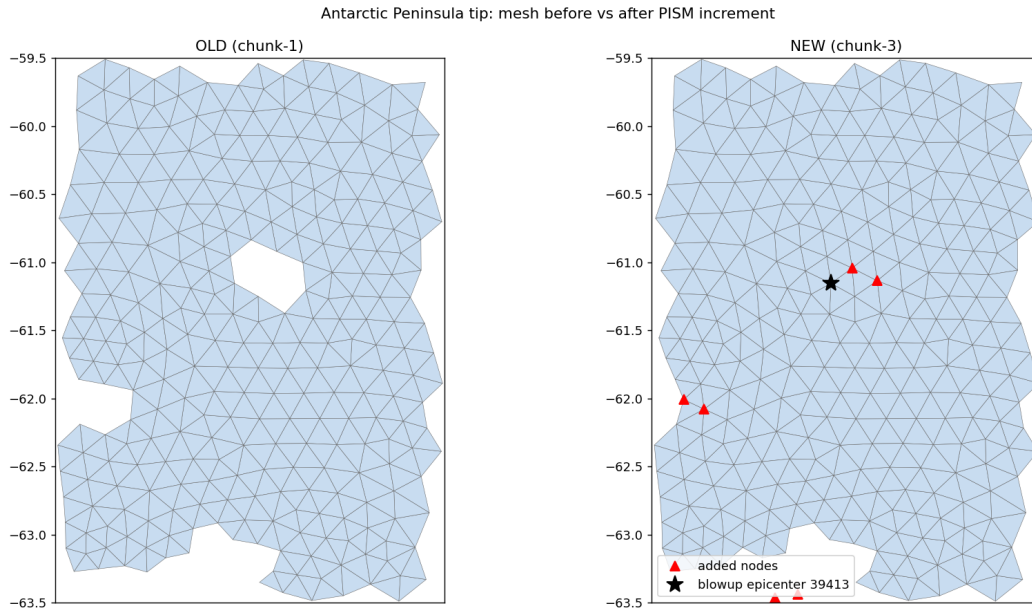
Figure 6: Bug VII. Left: the chunk-1 mesh has Elephant Island (the hole at 55.4°W, 61.1°S) and the Clarence/Gibbs notch. Right: after the PISM decade the bilinear mask remap has rounded both islands to ocean — the added nodes (red) fill them in, and the blowup epicenter (star) sits exactly on the drowned island.
