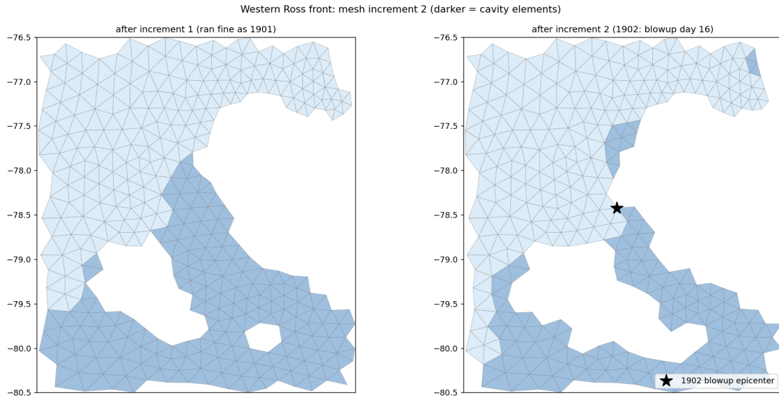
Figure 7: The second increment at the western Ross front (darker = cavity elements). Left: after increment 1 (ran a clean year as 1901). Right: after increment 2 — the front reorganizes, and the 1902 blowup epicenter (star) sits in a newly pinched notch between advancing and retreating ice.
