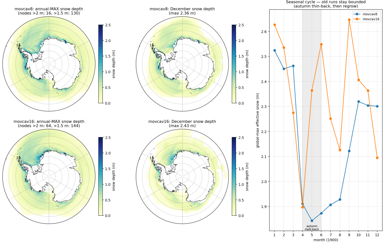
Figure 18: The extent of the coastal pile-up in the (pre-fix) movcav runs: annual-max and December snow depth, and the seasonal cycle. The thick snow is a band hugging the ice-shelf front (eastern Weddell/Fimbul, Amundsen), bounded at 2–2.6m by an autumn melt-back. Later runs that lost this melt-back drifted monotonically to 3.5 m — the insulation that raised Bug IV’s loop gain.
