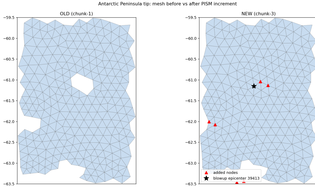
Figure 7: Bug VII. Left: the chunk-1 mesh has Elephant Island (the hole at 55.4^{\circ}\text{W} , 61.1^{\circ}\text{S} ) and the Clarence/Gibbs notch. Right: after the PISM decade the bilinear mask remap has rounded both islands to ocean — the added nodes (red) fill them in, and the blowup epicenter (star) sits exactly on the drowned island.
