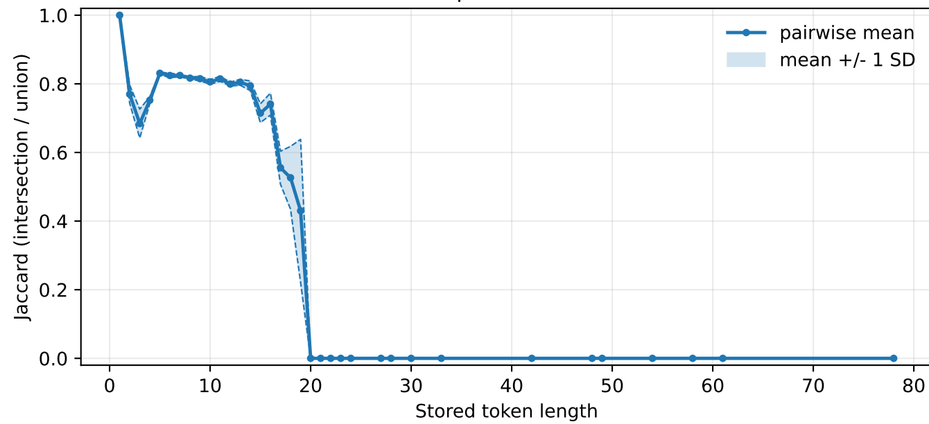
lp bias
