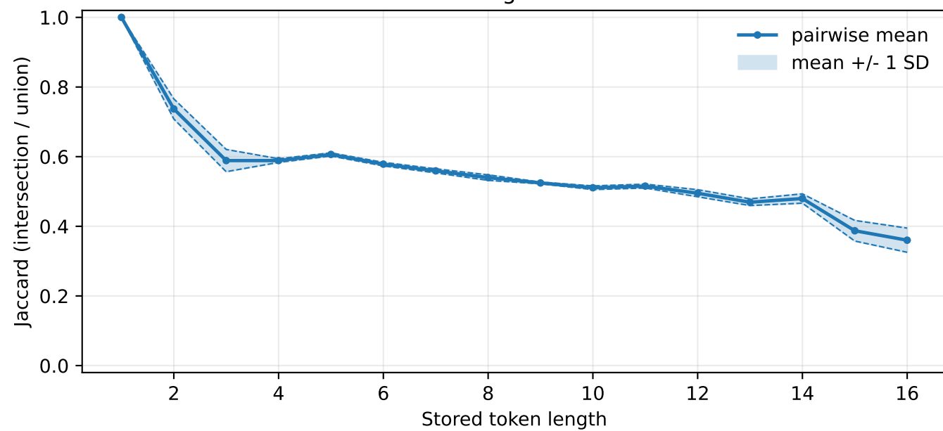
unigram
