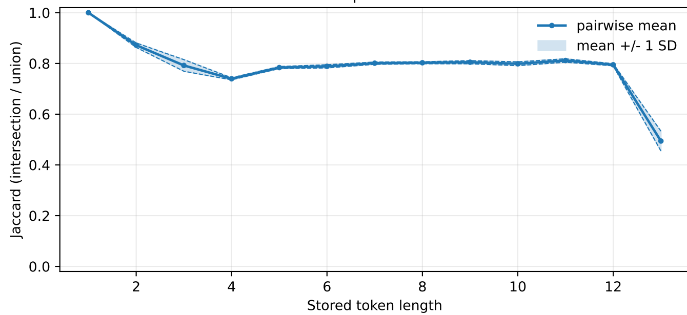
unigram
