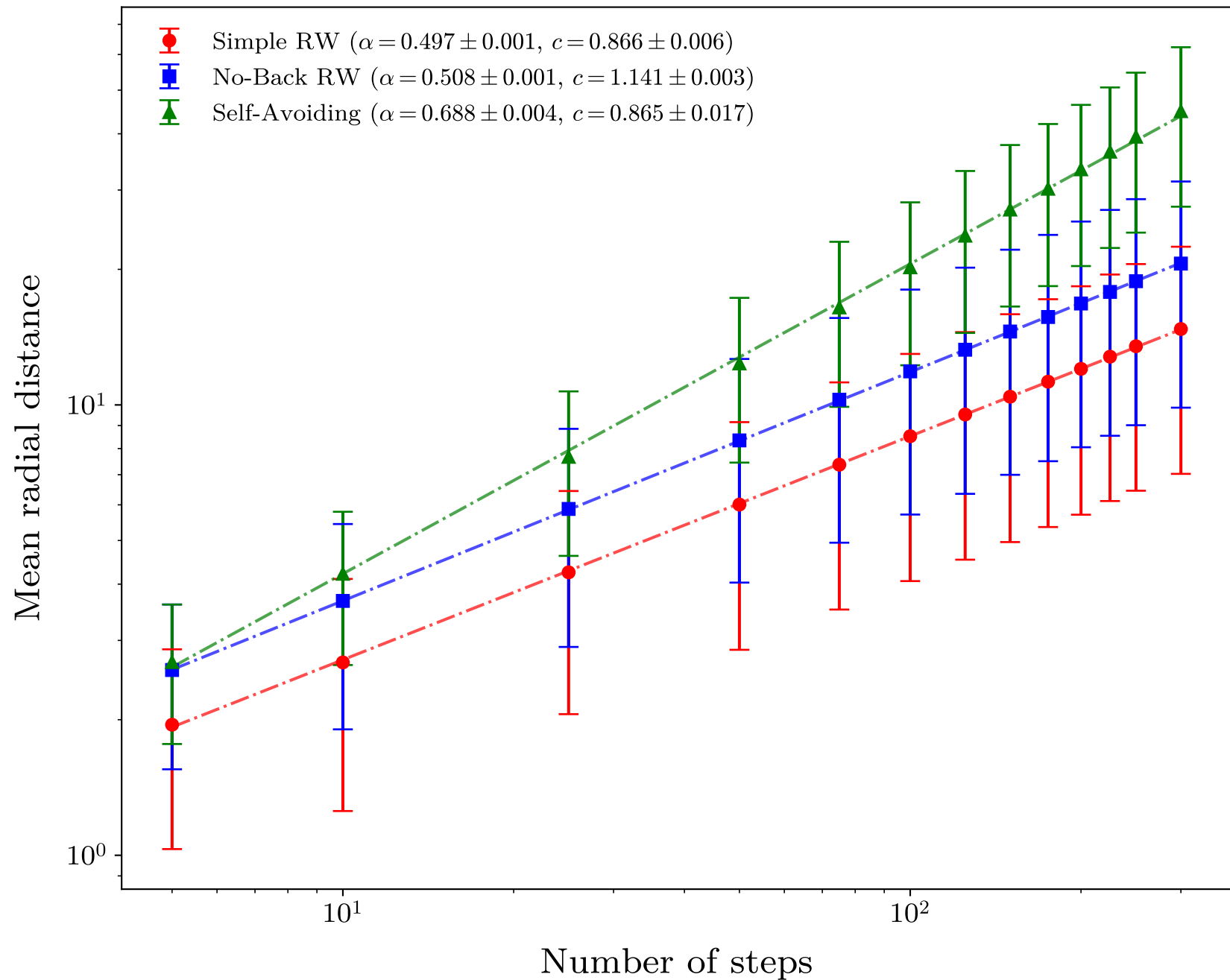
Log-Log plot of R vs. n on Penrose Tiling
