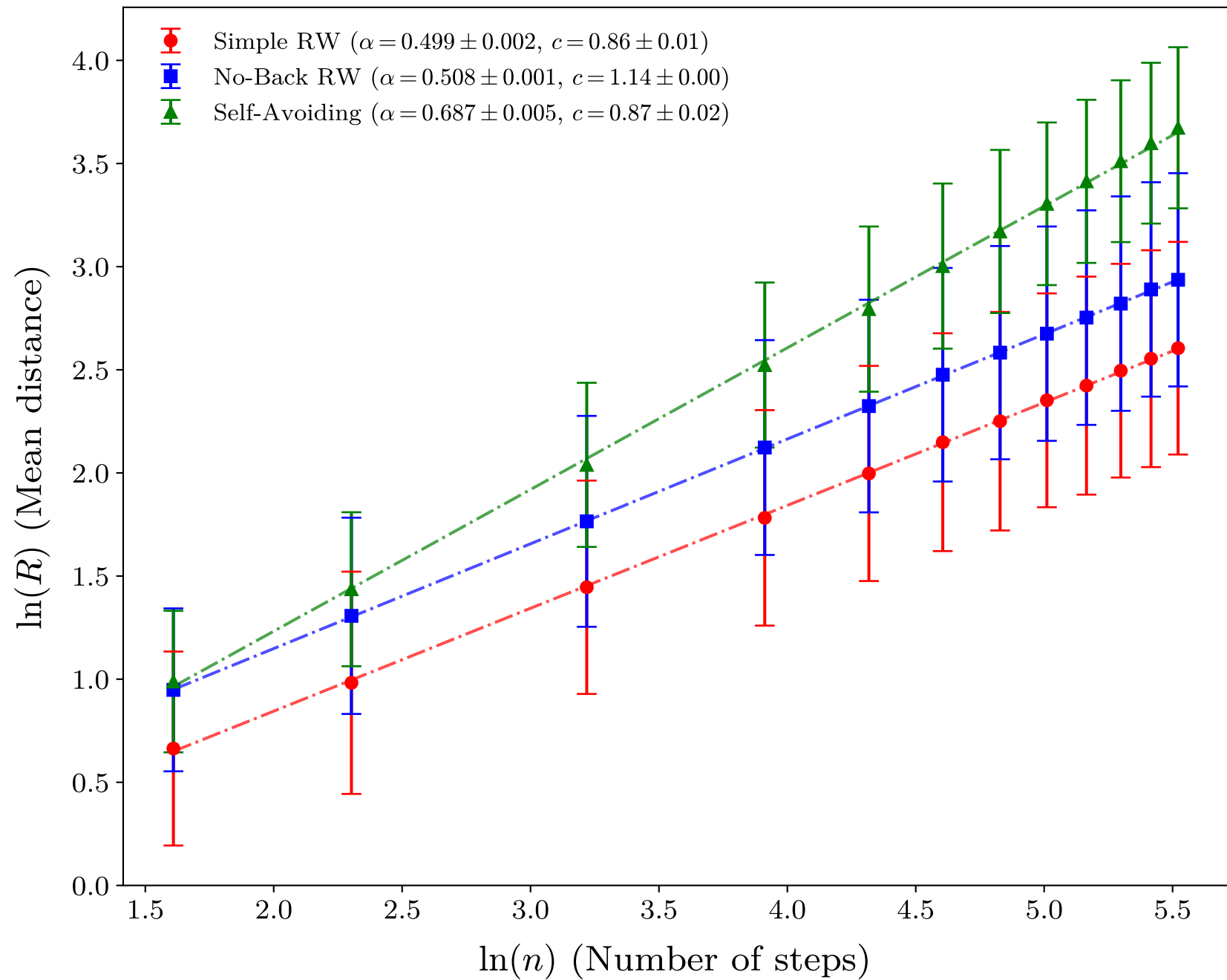
Log-Log plot of R vs. n (Penrose Tiling)
