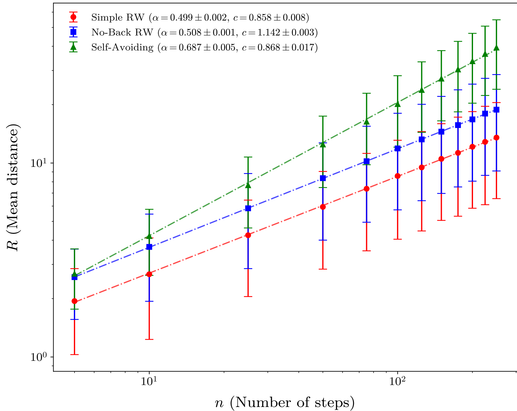
Log-Log plot of R vs. n (Penrose Tiling)
