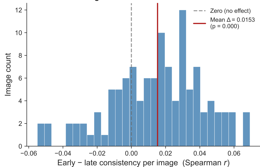
A Distribution of consistency differences between chronological halves
