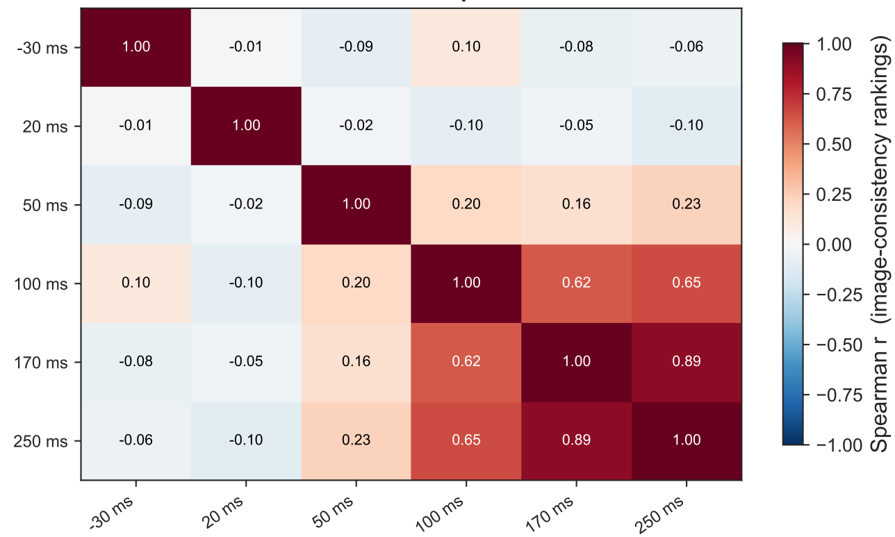
A Rank-correlation matrix across epochs
