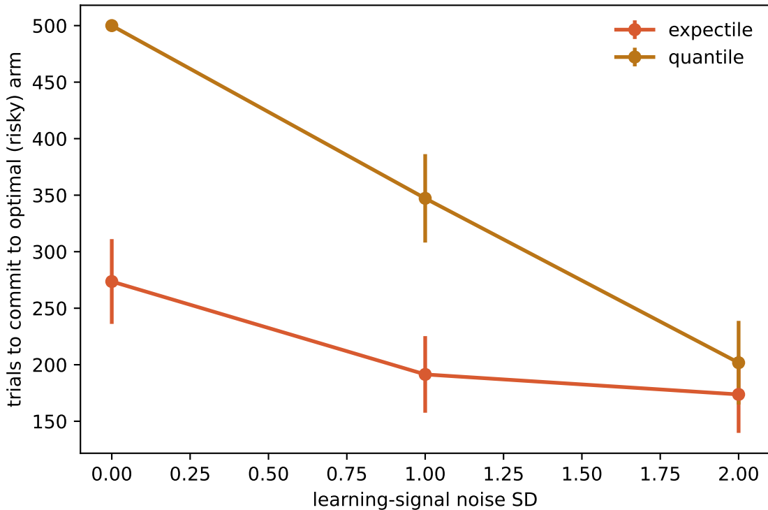
Task 3: Risk-sensitive survival time to identify optimal arm vs. noise
