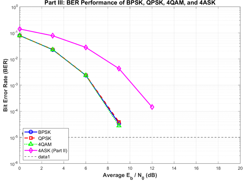
Figure 4: Part III: BER performance of BPSK, QPSK, 4QAM and 4ASK
