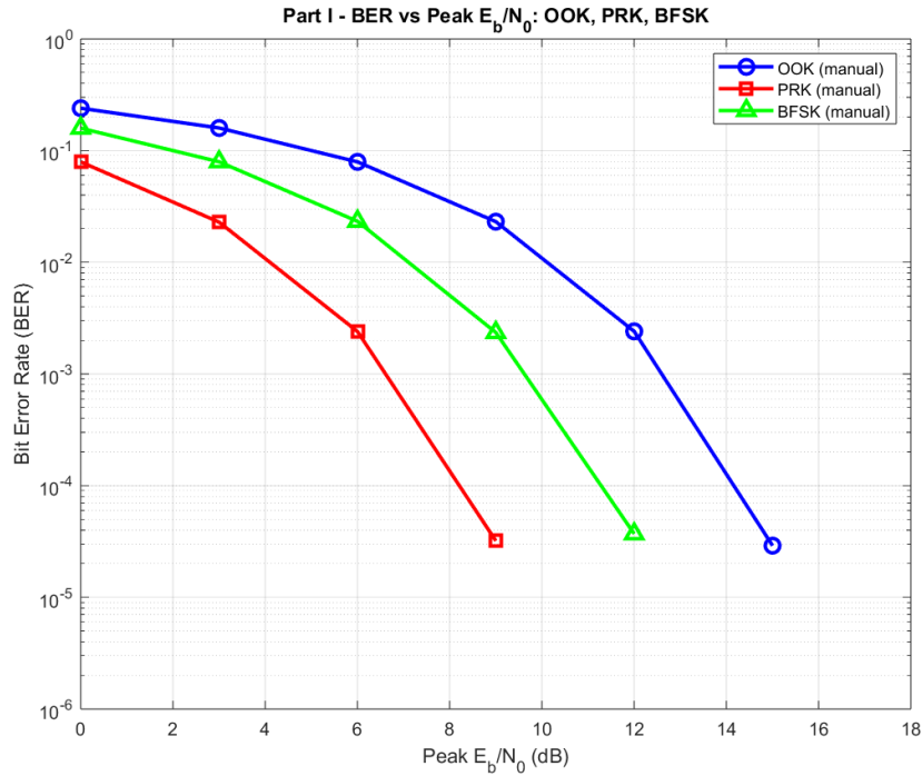
Figure 1: Probability of Error vs Peak E_b/N_0 (Manual Implementation)
