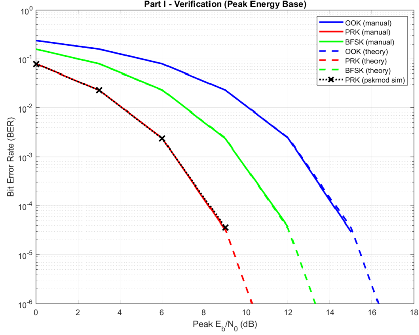
Figure 2: Probability of Error vs Peak E_b/N_0 (MATLAB Built-in Verification)
