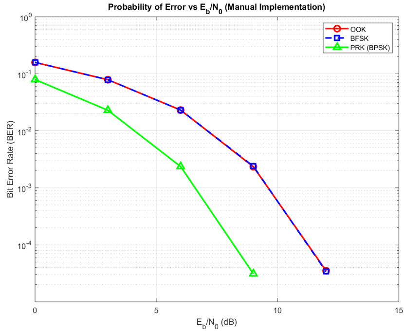
Figure 1: Probability of Error vs E_b/N_0 (Manual Implementation)
