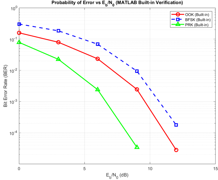
Figure 2: Probability of Error vs E_b/N_0 (MATLAB Built-in Verification)
