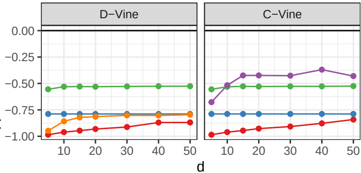
Approximation A3
