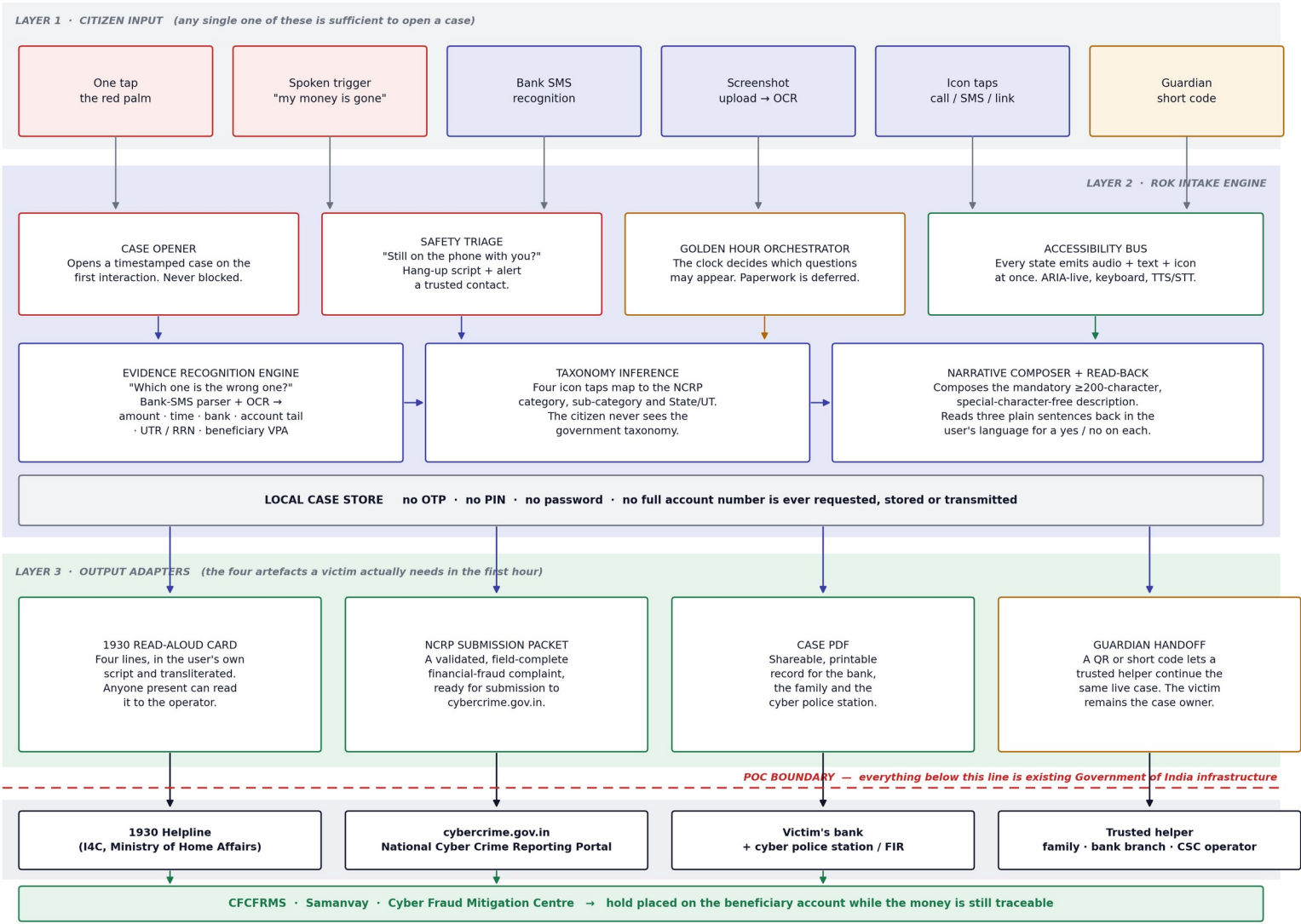
Figure 1 — Rok system architecture. Layers 1–3 are the browser-based proof of concept; everything below the dashed boundary is existing Government of India infrastructure.
