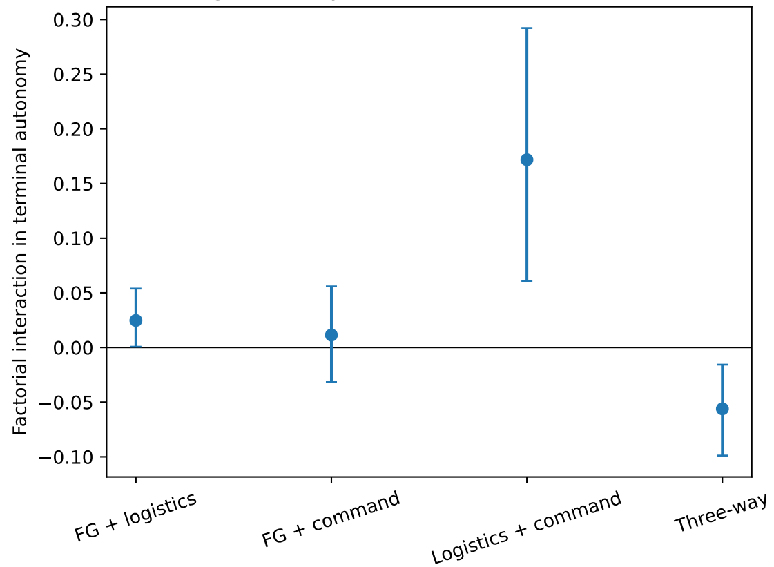
High-intensity nominal near-tie interactions
