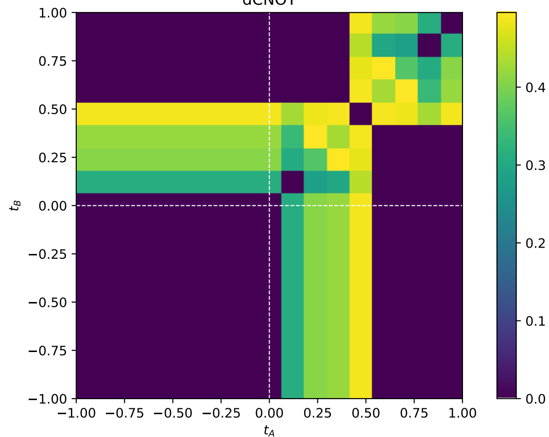
dCNOT
