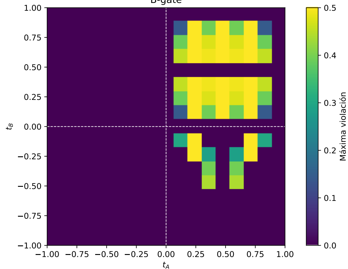
B-gate
