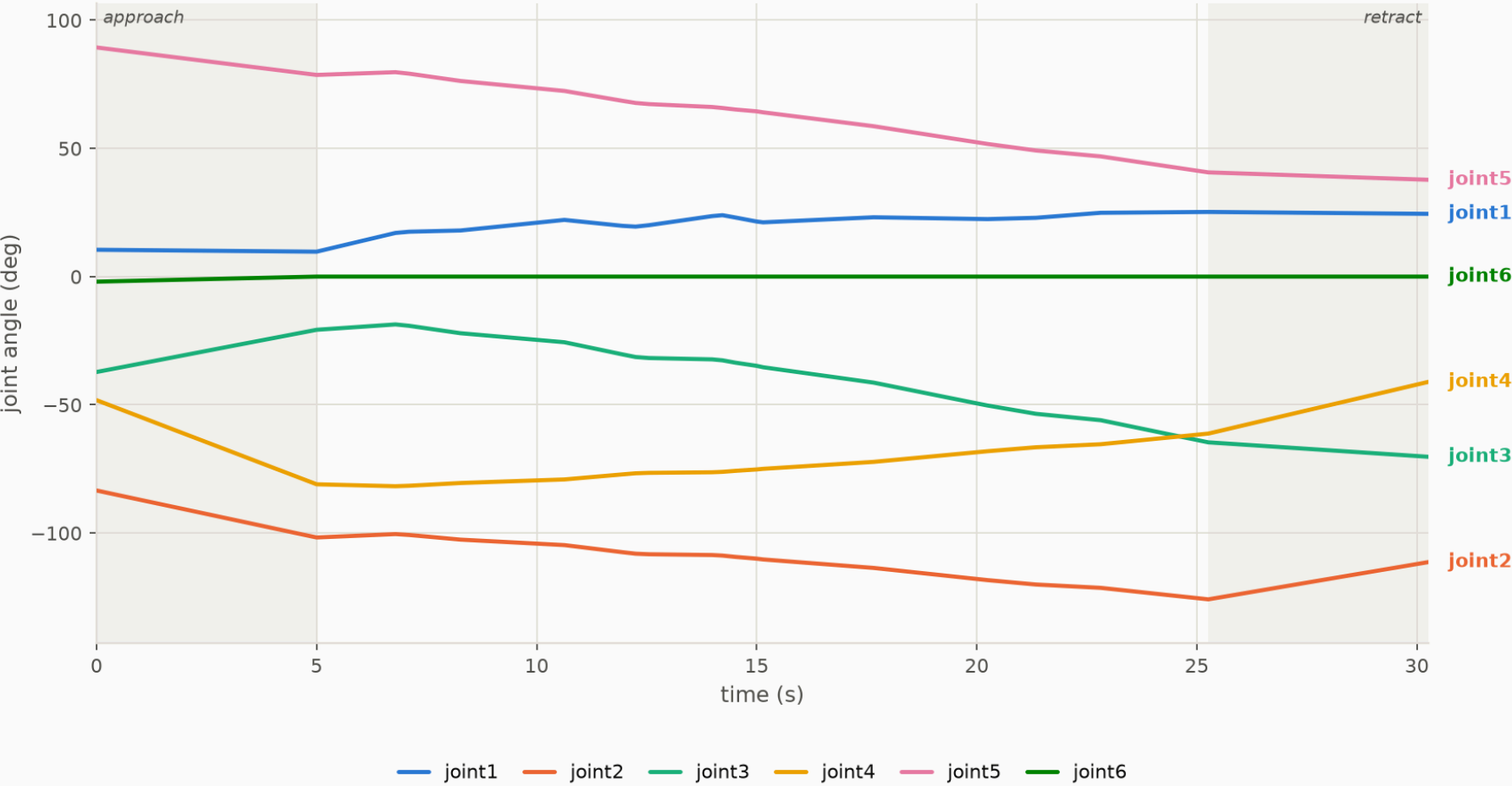
2 · SOLVED JOINT TRAJECTORY
