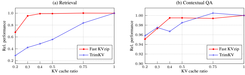
Figure 17: Comparison to TrimKV [5] with prefill-intensive tasks. We evaluate the official TrimKV model with Qwen3-4B-Instruct-2507 on retrieval and contextual QA tasks in Figure 9, and report the averaged scores. For each dataset, results are normalized with respect to full-cache performance prior to averaging. For Locret, the released models are outdated, and we replace performance comparisons with our analysis in Figure 5.
