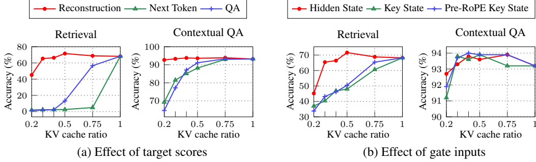
Figure 5: Gate Training Design Analysis. We evaluate gate training targets and inputs on Qwen2.5-7B-1M using a retrieval task (SCBench.KV) [31] and a contextual QA task (SQuAD) [40]. In (a), we compare different tasks to obtain target scores for gate training. For a fair comparison, we fix the gate architecture and only vary the task used to compute the maximum attention scores in our gate training (Figure 4). We use FineWeb-Edu for training data, except for QA where we use LongAlpaca [8] following Huang et al. [22].
