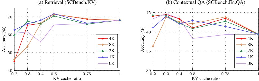
Figure 16: Effect of Local Window Size. We evaluate gates with a range of local window sizes, as described in Figure 2, using Qwen2.5-7B-1M. Note that our algorithm performs eviction that all configurations have an identical total KV cache size after eviction. In our main experiment, set the local window hyperparameter as 4K tokens for prefill and 128 tokens for decoding.
