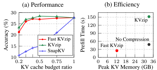
Figure 1: Highlighted results. (a) KV cache compression performance on OpenAI MRCC [37] compared to state-of-the-art methods using Qwen2.5-7b-1M [53]. (b) Chunked-prefill efficiency for 170K tokens on Qwen2.5-7b-14M (BF16 precision) with 30% KV cache budget.
