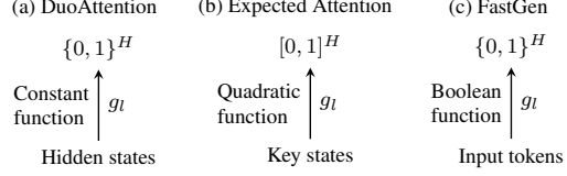
Figure 3: Gating formulation of existing KV compression methods at each attention layer. Note that we compare the core components of baseline methods, as each method jointly uses other techniques. For instance, FastGen combines its approach with cumulative attention scores [55].
