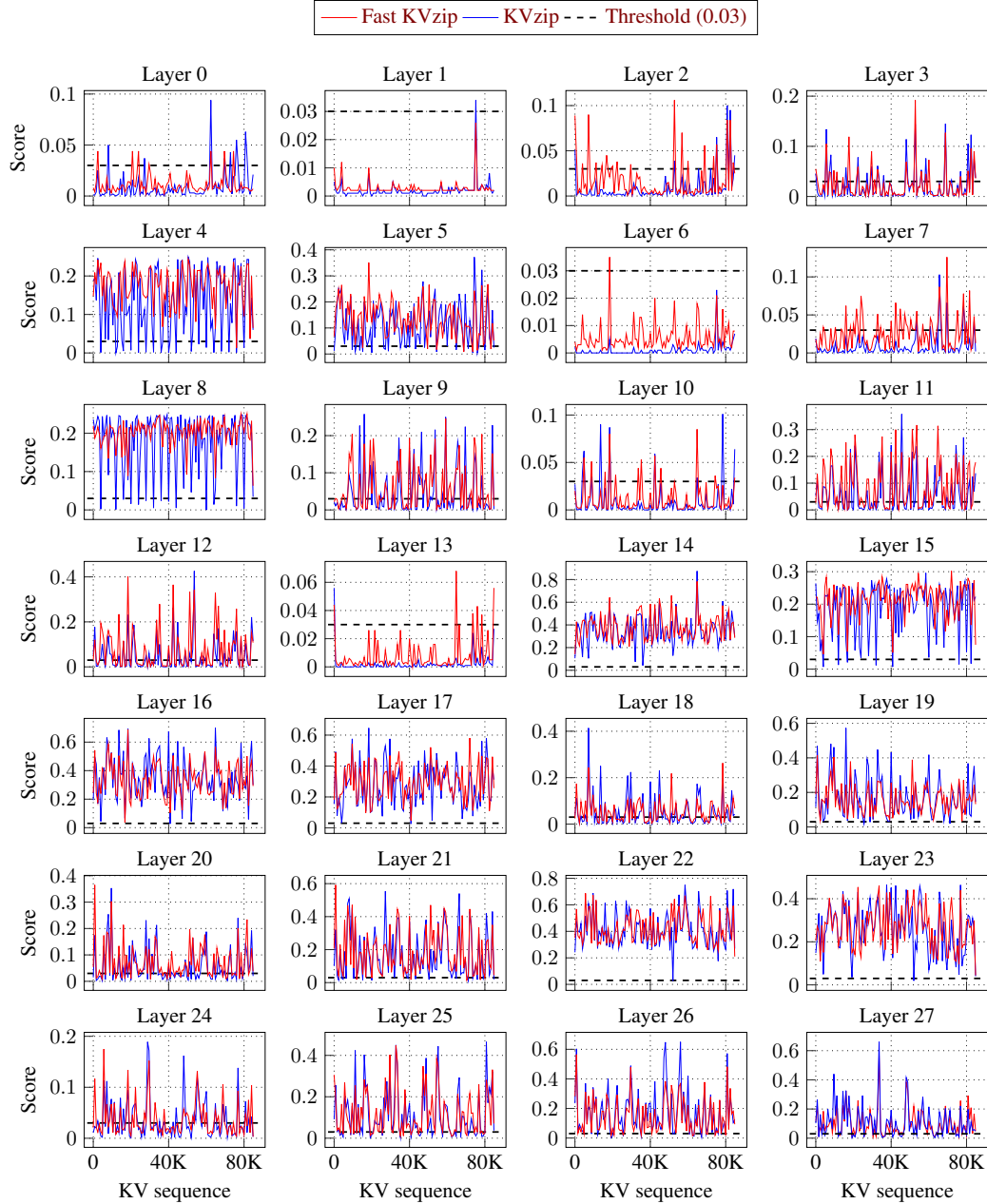
Figure 18: Prediction Comparison of Fast KVzip to KVzip. We use Qwen2.5-7B-1M with the SCBench.En.QA dataset, which were not used during training. For each layer, we plot the averaged score over heads. The dashed line represents the threshold value that results in a 36% KV cache budget ratio.
