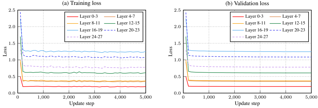
Figure 13: Gate training and validation loss trajectory per attention layer for Qwen2.5-7B-1M. We plot loss values averaged every four layers in the model.
