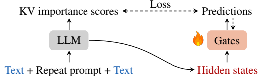
Figure 4: Gate training process. We compute the importance scores of KV pairs for a given text input following KVzip, which calculates the maximum attention score each KV pair receives during the context reconstruction [26]. We train gating modules to predict these scores from the corresponding input hidden states at each attention layer given the text. Please refer to Section A for further details and the training hyperparameters.
