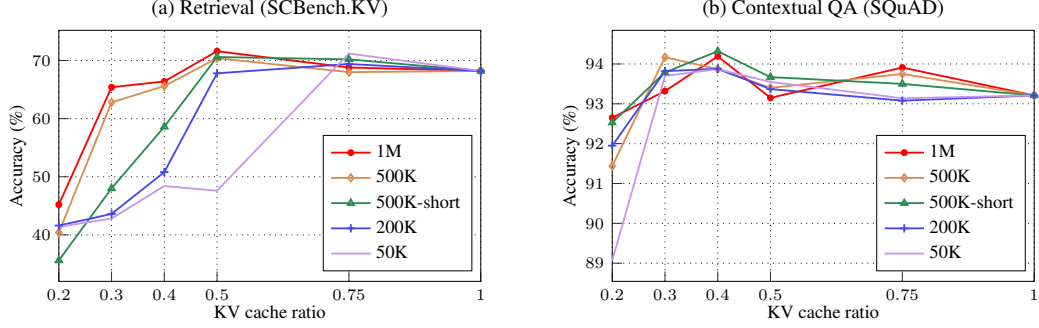
Figure 14: Effect of Training Data Size. We evaluate gates trained with different amounts of training data sampled from FineWeb-Edu using Qwen2.5-7B-1M. For the other settings, we uniformly reduce the context lengths of the data.
