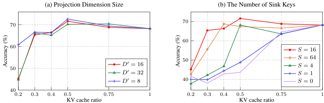
Figure 15: Effect of Gate Configuration. We evaluate gates with different numbers of sink keys S and projection dimensions D' using Qwen2.5-7B-1M on SCBench.KV.
