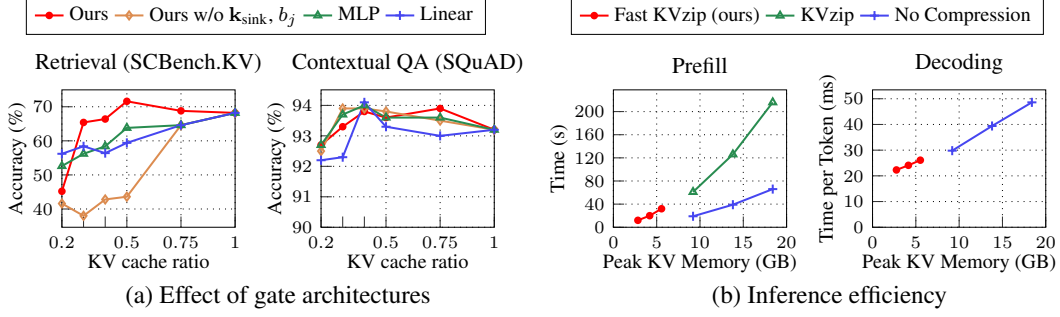
Figure 7: (a) Architecture analysis. We compare our sink-attention, a variant without learnable denominator terms, a two-layer MLP, and a linear model, using Qwen2.5-7B-1M. For a fair comparison, we equalize the number of parameters across all architectures. (b) Prefill and decoding efficiency of the Qwen2.5-7B-1M model using a 30% KV budget ratio with PyTorch and FlashAttention-2 [13] on a single H100 GPU. Points in the plot correspond to context lengths of 160K, 240K, and 320K. In Section B.3, we provide an end-to-end latency analysis.
