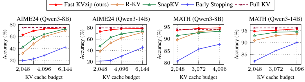
Figure 11: Decoding-intensive tasks. For AIME24, we averaged scores over 16 random seeds.
