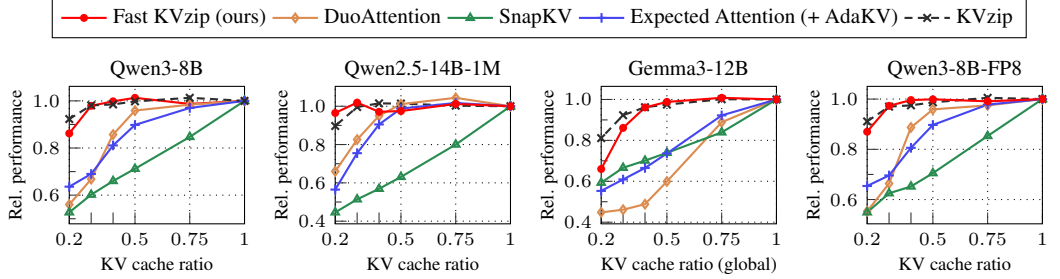
Figure 10: Performance across different models , averaged over 12 benchmark datasets. For each dataset, results are normalized with respect to full-cache performance prior to averaging.
