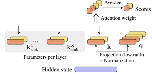
Figure 8: Gate architecture. We propose a sink-attention architecture using a fixed set of keys per layer. Given a hidden state \mathbf{h} \in \mathbb{R}^D , we compute the importance scores of KV as \mathbf{s} \in [0, 1]^H .
