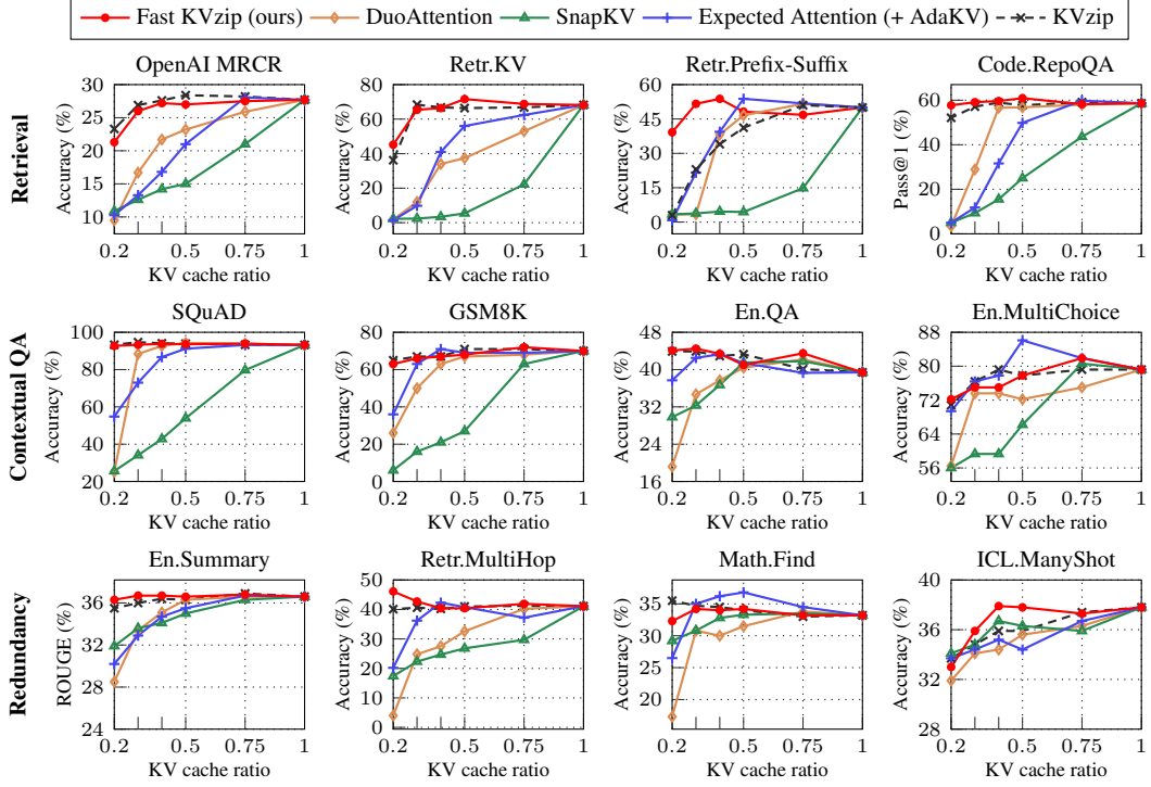
Figure 9: Prefill-intensive benchmark results with Qwen2.5-7B-1M under varying KV cache budget ratios from 0.2 to 1.0. Tasks are organized into three categories: (1) retrieval-intensive, (2) contextual understanding, and (3) high context redundancy.
