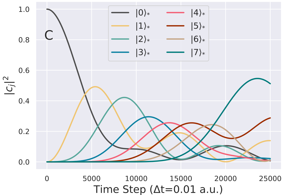
Exciton Transfer (8-Ethylene Chain)
