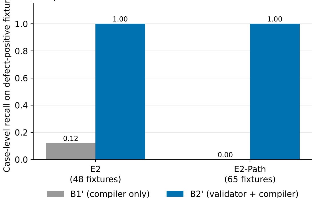
Static validator recall vs. compiler-only baseline (component-level conformance, not end-to-end LLM eval)
