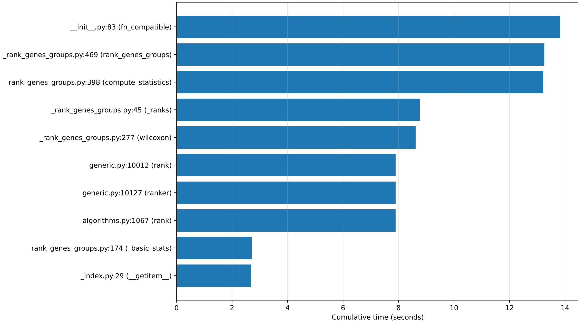
pbmc10k: top rank_genes_groups functions
