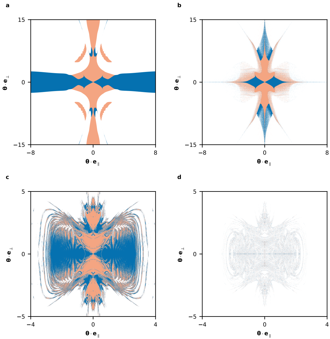
Extended Data Fig. 9. Metamorphoses of riddling. Destination maps for initializations in the same two-dimensional slice of parameter space as Fig. 3. Only the learning rate \eta is varied; all other settings are held fixed. a , At \eta = 0.1 , there is no riddling. b , At \eta = 1 , there is pseudo-riddling, which is a mixture of open and riddled sets. c , At \eta = 2.7 , there is true riddling but the exact structure is different to Fig. 3b. d , At \eta = 3 , the time-dependent basin of a chaotic transient is riddled with diverging initializations. See Supplementary Sec. 1 for further information on these regimes.
