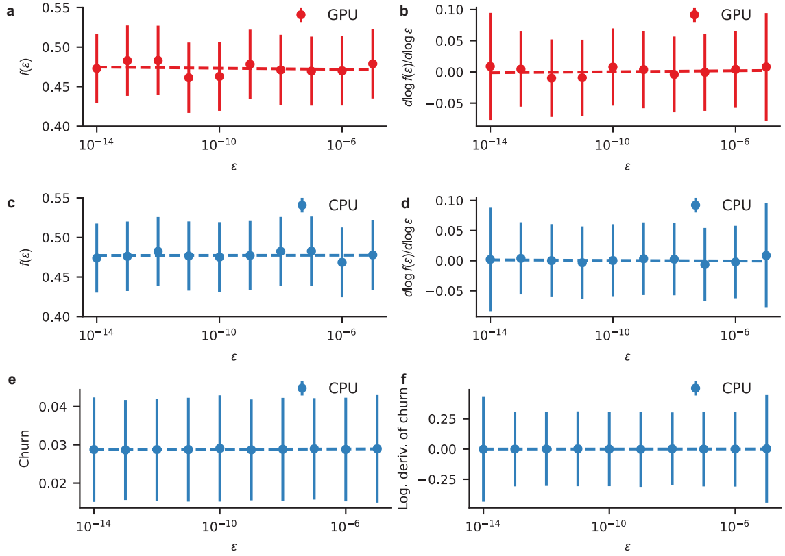
Fig. 5. Parameter- and function-space uncertainty exponents. a , The uncertainty fraction f(\epsilon) for initializations within a \epsilon -hypercube centered at the middle of Fig. 4d, (\theta \cdot e_{\parallel}, \theta \cdot e_{\perp}) = (16.0005, 0.0355) . Networks are trained on GPU, which is faster than CPU but non-deterministic. Dots and error bars show the mean and 95% confidence intervals from 10^4 bootstrap resamples, each of size n = 500 \epsilon -close pairs. A power-law fit f(\epsilon) \propto \epsilon^{\phi_p} (dashed line) yields the uncertainty exponent \phi_p = 0.000 \pm 0.002 . b , The logarithmic derivative of (a). c , Same as (a), except with CPU training to ensure determinism. The uncertainty exponent is also \phi_p = 0.000 \pm 0.002 . d , The logarithmic derivative of (c). e , Dots and error bars denote the mean churn and 95% confidence interval across n = 250 CPU-trained \epsilon -close pairs. The functional uncertainty exponent using churn is \phi_f = 0.00 \pm 0.01 and the mean churn plateaus at approximately 2.9%. f , The logarithmic derivative of (e).
