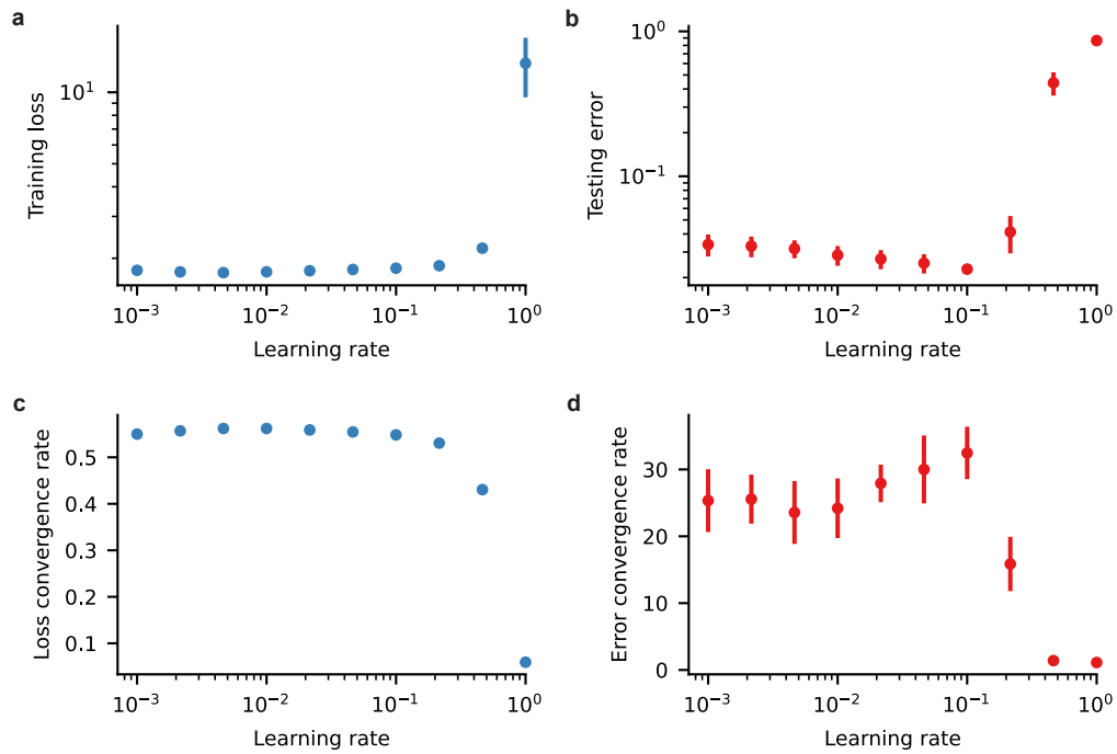
Extended Data Fig. 8. Learning-rate sweep. Dots and error bars show the mean and 95% confidence interval across n = 5 independent 100-epoch training runs on randomly initialized VGG-12 networks. a , Minimum training loss achieved during training. b , Minimum testing error achieved during training. c , Loss convergence rate defined as \sum_t \bar{L}_t^{-1} , where \bar{L}_t denotes the average training loss in the t -th epoch. The larger the value, the longer the training spends with lower loss. d , Error convergence rate defined analogously using the testing error. Note that the generalization metrics in (c) and (d) are optimal at \eta = 0.1 .
