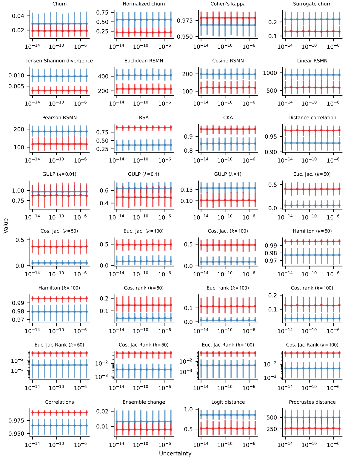
Extended Data Fig. 3. Scale-insensitive functional similarity measures. Each of the 32 measures defined in Supplementary Sec. 5 is evaluated within the riddling-like regime (blue, \eta = 0.1 ) and outside of it (red, \eta = 0.001 ). Dots and error bars denote the mean and 2.5-to-97.5 percentile range computed from n = 250 \varepsilon -close pairs for each uncertainty scale \varepsilon . Outside the riddling-like regime, there are substantially smaller functional and representational differences across all measures, indicating markedly higher reproducibility (see Supplementary Sec. 6 for details).
