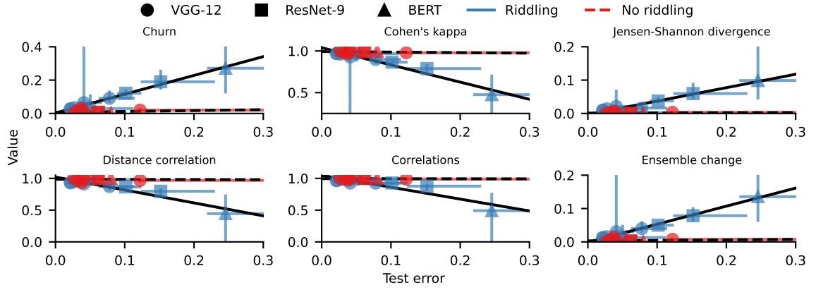
Extended Data Fig. 4. Diagnostic for riddling-like behaviors based on functional similarity measures. Mean functional similarity is visualized as a function of the mean test error within the riddling-like regime (blue, labeled “riddling”) and outside of it (red, labeled “no riddling”) across all experimental configurations. Each experimental configuration is labeled by a code: VGG-main, VGG-nln, VGG-bias, VGG-ReLU, Res-SGD, Res-AdamW, BERT (see Supplementary Sec. 8 for details of these experiments). Error bars denote the 2.5-to-97.5 percentile range for both similarity values and test errors. The sample size is n = 50 for VGG-bias, Res-SGD, BERT, Res-AdamW; n = 75 for VGG-GD; n = 250 for VGG-main, VGG-nln, VGG-ReLU, VGG-L1. Error bars exceeding the axis limits are clipped for visual clarity. In the riddling-like regime, functional similarity and generalization exhibit a linear trend (solid black line). Outside this regime, functional differences are negligible, independent of generalization (dashed black line). See Supplementary Sec. 6 for further details, including fitted parameters.
