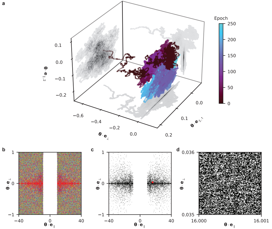
Fig. 4. Riddling-like dynamics of deep neural network training. a , A randomly initialized VGG-12 network is attracted to a parity-invariant subspace during training. The vectorized network weights \Theta are projected onto three random dimensions: \mathbf{e}_{||,1} , \mathbf{e}_{||,2} (longitudinal to the invariant subspace) and \mathbf{e}_{\perp} (transverse). The shadow on each pane is a two-dimensional histogram, where darker shades indicate higher frequency. b , Training destination map for a 255 \times 255 uniform grid of initializations on the plane spanned by \mathbf{e}_{||} = \mathbf{e}_{||,1} and \mathbf{e}_{\perp} . Each color denotes a unique parity-invariant subspace; in total, there are 1772 different destinations. White points approach the origin. c , Same as (b), except initializations converging to the invariant subspace at \Theta \cdot \mathbf{e}_{\perp} = 0 are colored black. All other destinations are white. d , Magnification around the red dot in (c) on a 128 \times 128 grid.
