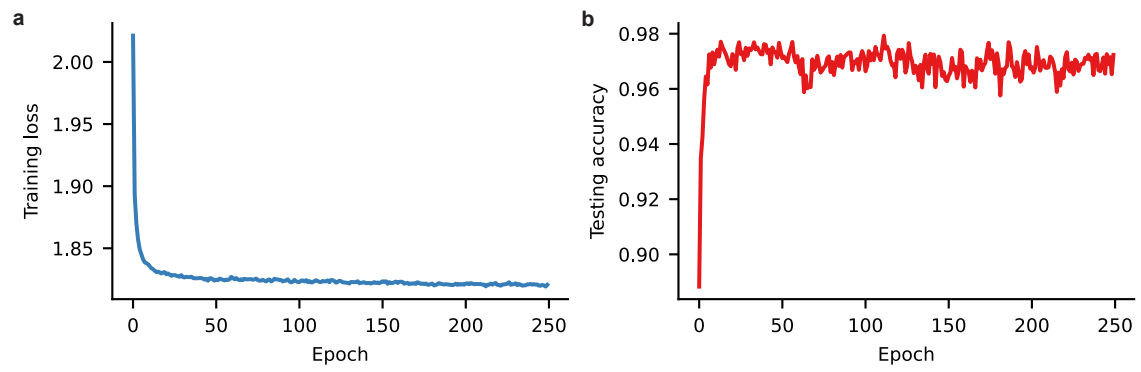
Extended Data Fig. 10. Learning curves. a , Loss on the training dataset at each epoch of training the randomly initialized VGG-12 network in Fig. 4a. b , Same as (a), except with the accuracy on the testing dataset.
