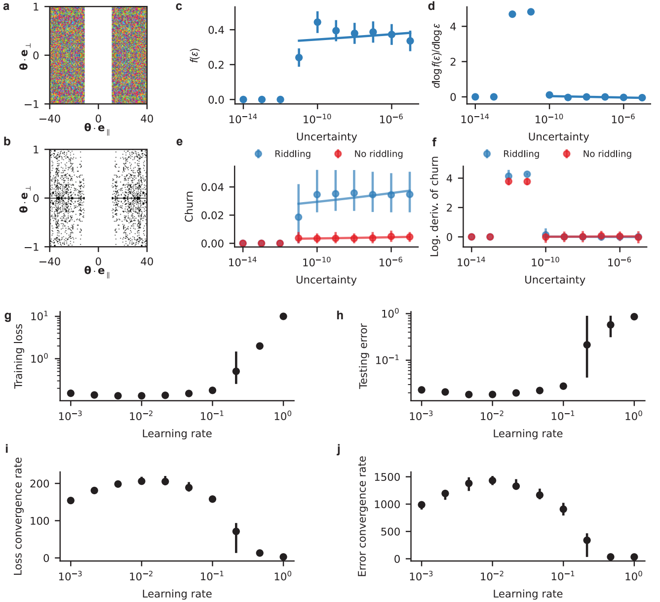
Extended Data Fig. 5. Riddling analysis for training without label noise. Riddling analysis is applied to a VGG-12 network, identical to the one used in Figs. 4 and 5, trained to classify MNIST without label noise; see Supplementary Sec. 8 for full details. a , Parameter-space destination map on a 127 \times 127 grid. b , Same as (a), except initializations converging to the permutation-invariant subspace at \theta \cdot \mathbf{e}_{\perp} = 0 are colored black. All other destinations are white. c , The uncertainty fraction f(\varepsilon) for initializations within a \varepsilon -hypercube centered at (\theta \cdot \mathbf{e}_{\parallel}, \theta \cdot \mathbf{e}_{\perp}) = (26, 0.1) . Networks are trained on CPU. Dots and error bars represent the mean and 95% confidence interval across n = 250 \varepsilon -close pairs for each uncertainty \varepsilon . A power-law fit f(\varepsilon) \propto \varepsilon^{\phi_p} (solid line) yields the uncertainty exponent \phi_p = -0.003 \pm 0.007 . d , The logarithmic derivative of (c). e , Dots and error bars represent the mean churn and 2.5-to-97.5 percentile range across n = 250 \varepsilon -close pairs for each \varepsilon in the riddling-like regime (blue, labeled “riddling”; \eta = 0.1 ) and outside of it (red, labeled “no riddling”; \eta = 0.001 ). In the riddling-like regime, the churn is significant (3.5% on average, before suddenly dropping to zero at small initialization uncertainty due to floating point errors; see Supplementary Sec. 8) and shows little improvement as uncertainty \varepsilon is reduced by 6 orders of magnitude ( \phi_f = 0.02 \pm 0.01 ). Outside this regime, the churn is practically insignificant (approximately 0.4%). f , The logarithmic derivative of (e). g , Dots and error bars show the mean and full range of training loss across n = 5 independent 30-epoch training runs. h , Testing error. i , Loss convergence rate, defined as \sum_t \bar{L}_t^{-1} where \bar{L}_t denotes the average training loss in the t -th epoch. j , Error convergence rate defined analogously using the testing error. This training configuration does not exhibit a performance-reproducibility trade-off as riddling-like irreproducibility does not coincide with optimal performance.
