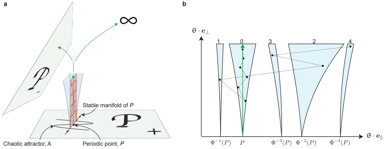
Extended Data Fig. 2. Schematic of the mechanism for riddling. a , A transversely unstable periodic point P is embedded in the chaotic attractor A \subset \mathcal{P}_+ . Around the stable manifold (orange area) of a heteroclinic trajectory (green arrows), there exists a hyperwedge of initializations (blue volume) whose orbits leave A and either converge to the attractor in \mathcal{P}_- or diverge to infinity. b , The hyperwedge anchored at the periodic point P is labeled 0. Initializations within its pre-images are also ejected away from \mathcal{P}_+ . For example, the dots and dashed line depicts the trajectory of an initialization starting within the fourth pre-image of the hyperwedge (labeled 4); it travels across the pre-images until it reaches the original hyperwedge, where it follows the heteroclinic trajectory to the competing outcome. These pre-images constitute a dense set of hyperwedges anchored at the pre-iterates of P , denoted \Phi^{-m}(P) , which are dense in the attractor A .
