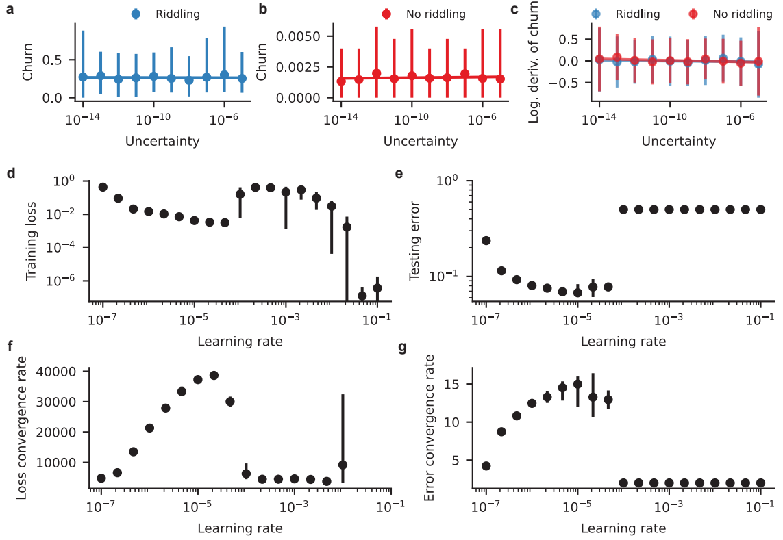
Extended Data Fig. 6. Riddling analysis for BERT fine-tuning. A pre-trained BERT transformer [37] is fine-tuned to perform sentiment classification on the IMDB dataset. Its final state is used as the reference point for functional analysis. See “Methods” for further details on the experimental configuration. a , At the near-optimal learning rate of \eta = 5 \times 10^{-5} , churn is significant (27% on average) and shows no improvement as uncertainty \varepsilon is reduced by 10 orders of magnitude ( \phi_f = -0.001 \pm 0.004 ), which is evidence for riddling. Dots and error bars represent the mean and 2.5-to-97.5 percentile range across n = 50 \varepsilon -close pairs for each uncertainty \varepsilon . b , Same as (a), except at the sub-optimal learning rate of \eta = 10^{-7} . The churn is negligible (i.e., learned functions are essentially identical; 0.1% on average), analogous to f(\varepsilon) = 0 for a non-riddled basin. The churn magnitude is the main distinction between inside and outside the riddling-like regime (Supplementary Sec. 6). c , Logarithmic derivatives of the trends in (a) and (b), showing the functional uncertainty exponent remains near-zero at small scales. d , Dots and error bars show the mean and full range of training loss across n = 5 independent fine-tuning runs. e , Testing error. f , Loss convergence rate. g , Error convergence rate.
