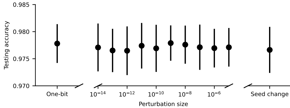
Extended Data Fig. 7. Model variability is insensitive to perturbation size. Dots and error bars show the mean and standard deviation of the testing accuracy across n = 100 30-epoch training runs with varying perturbations. The first point represents a flip to the least significant bit of a randomly selected parameter of the reference network in Fig. 5. The middle points apply random perturbations to each parameter of the reference network by a uniform random value U(-\varepsilon, \varepsilon) , where \varepsilon is the perturbation size. The final point uses random Kaiming-initializations [70] with different seeds.
