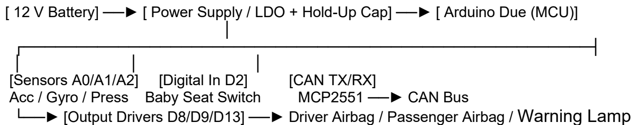
Figure 3.2 Hardware Architecture Block Diagram [1][12]
