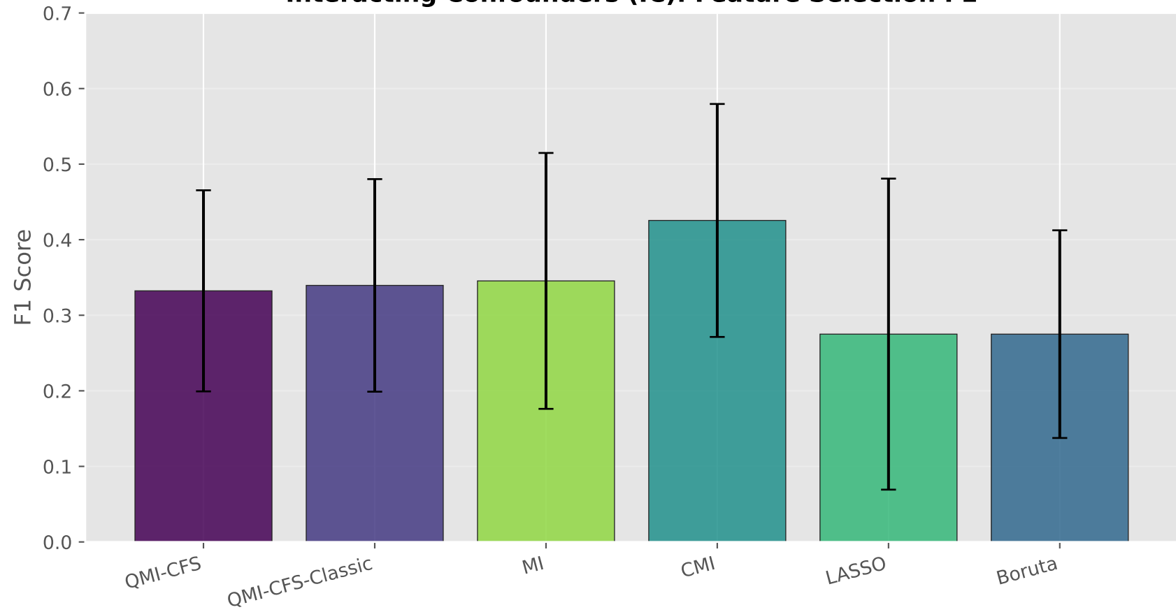
Interacting Confounders (IC): Feature Selection F1
