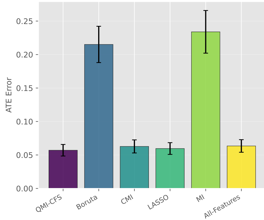
IHDP: ATE Error by Method
