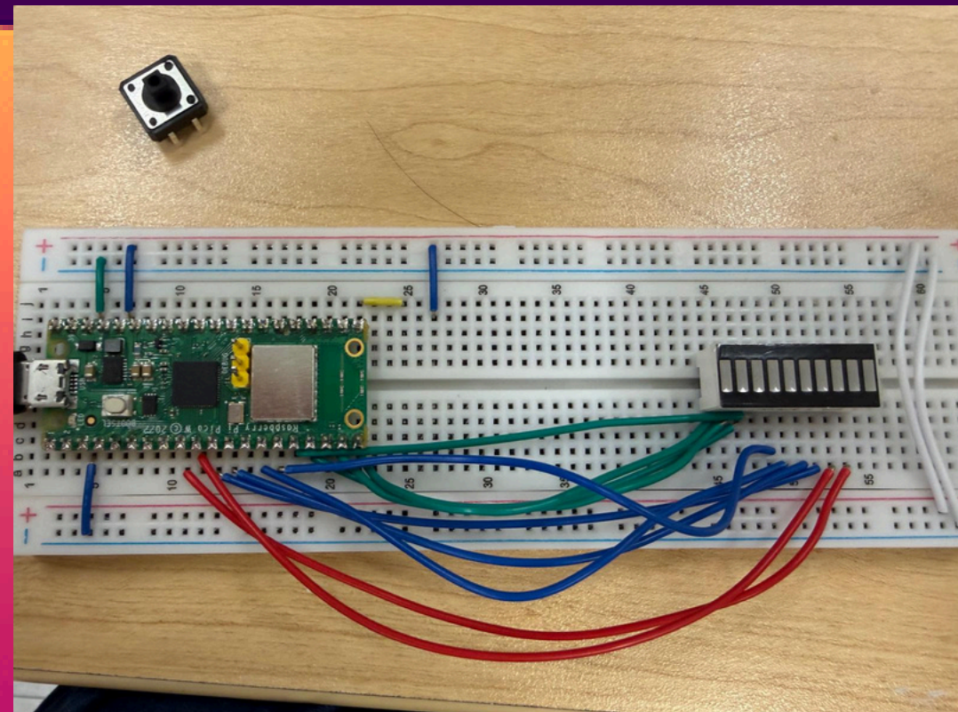
HOOK UP YOUR LED BAR GRAPH
