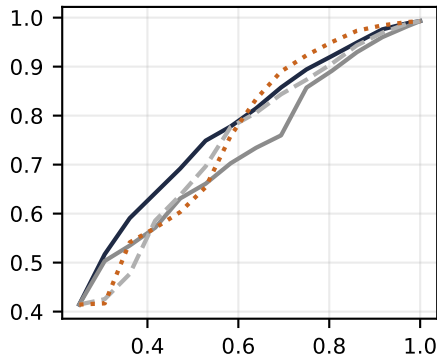
PbLa
