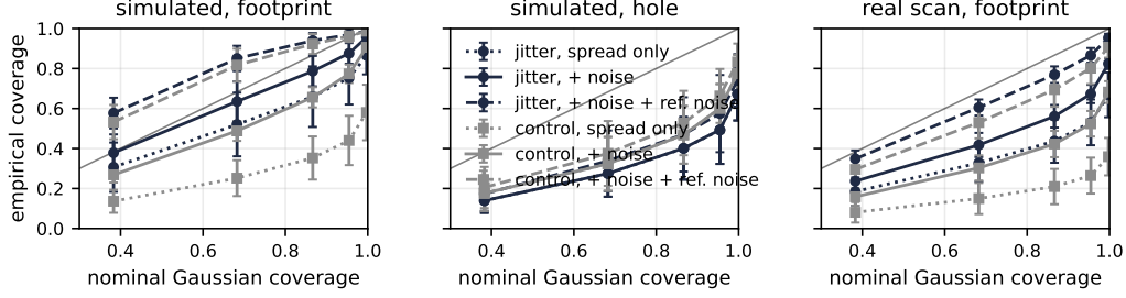
Figure 1: Coverage of |\text{mean} - \text{truth}| \leq z\sigma vs the Gaussian target, jitter (navy) and control (grey); dotted: spread only, solid: plus propagated noise, dashed: plus reference-map noise (sim upper bound; the correct band on the real scan). Bars: sd over lines and cases. Left: 32 simulated cases (footprint); middle: in a 14 \times 20 hole; right: the real scan.
