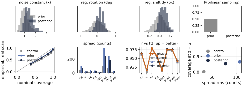
Figure 3: Top: prior (grey) and posterior (navy) ABC marginals from one real scan, for the knobs the data moves (gain slope and angle match the prior; omitted); P(\text{bilinear}) drops from 0.5 to 0.000. Bottom: real-scan calibration, per-line spread and r (physics in orange), and the coverage-vs-width tradeoff.
