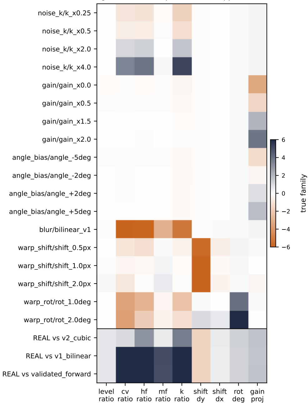
signature: mean z per statistic (clipped at \pm 6 )
