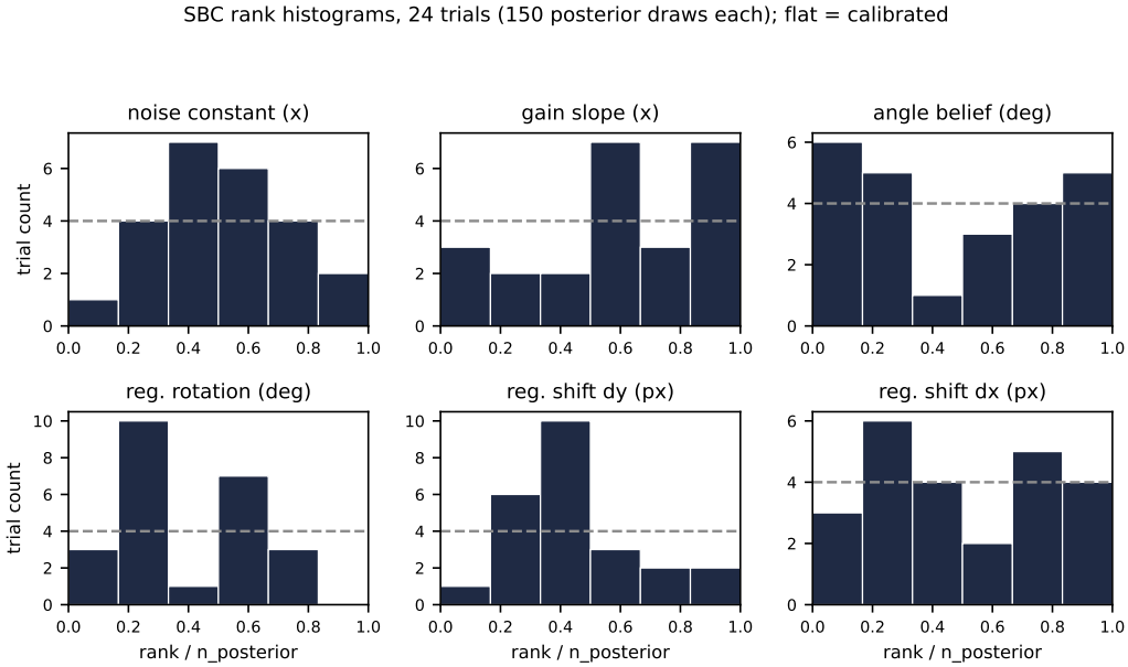
Figure 5: Simulation-based calibration [10]: rank of the true knob value inside 150 posterior draws, over 24 trials with known ground truth (flat = calibrated).
