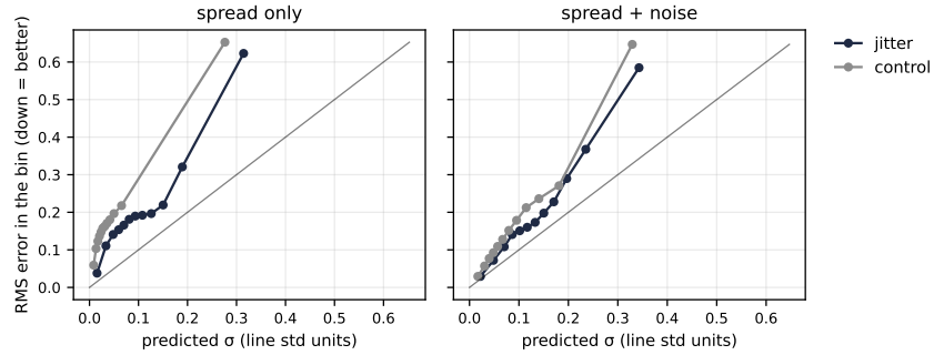
Figure 7: Binned reliability: RMS error against predicted \sigma in twelve \sigma -quantile bins, pooled over simulated cases and lines in units of each line's standard deviation; diagonal = calibrated. Left: ensemble spread only; right: spread plus propagated noise.
