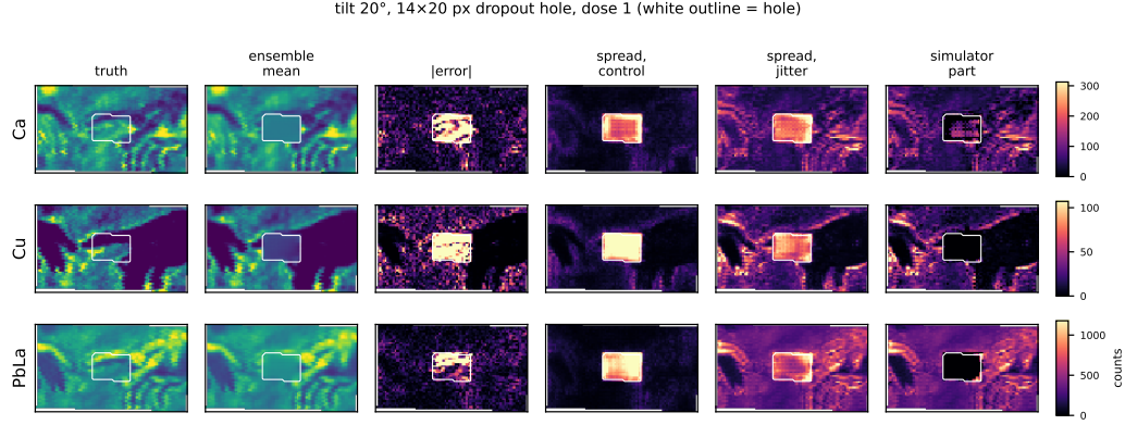
Figure 6: Spread maps on the harsh case (20°, 14 × 20 hole, white outline), three lines. Columns: reference, jitter-ensemble mean, absolute error, control spread, jitter spread, and the simulator part \sqrt{\max(\sigma_{\text{jitter}}^2 - \sigma_{\text{control}}^2, 0)} ; the three spread panels of a line share one colour scale. The control spread lives in the hole; the jitter spread follows the painting's structure; inside the hole the jitter ensemble is narrower than the control (dark).
