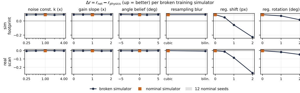
Figure 2: Defect tolerance: r(\text{net}) - r(\text{physics}) (up = better), one network per broken training simulator, on nominal simulated cases (top) and the real scan (bottom); grey band: 12 nominal seeds; orange: nominal. The hole region is omitted (seed band [-0.03, +0.27] , no tolerance signal). Geometry is the cliff; blur is visible only on the real scan.
