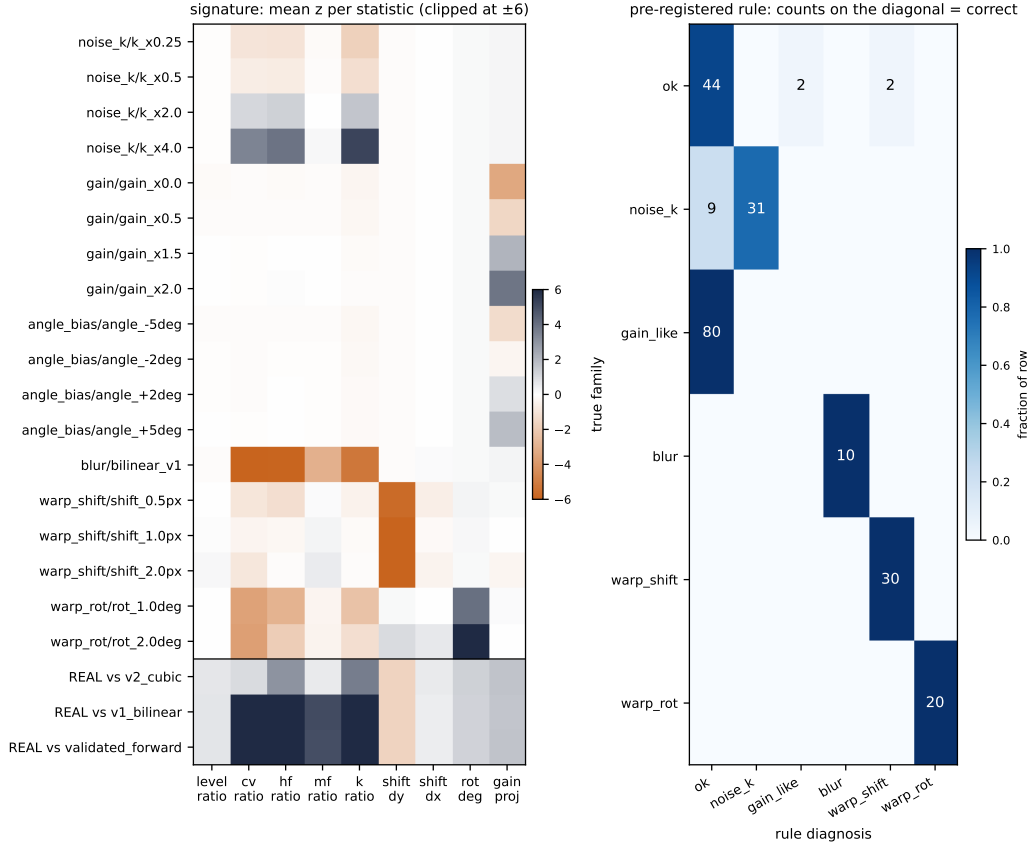
Figure 8: Blind diagnostics. Left: signature of every defect rung, the mean z of each statistic against the calibration-uncertainty null (both test angles pooled, clipped at \pm 6 ); the bottom block is the real scan against three simulators (v2 cubic, v1 bilinear, validated bilinear emulator). Right: identification counts of the pre-registered rule, true family (grouped) versus diagnosis.
