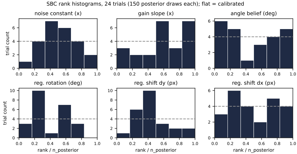
Figure 5: Simulation-based calibration [10]: rank of the true knob value inside 150 posterior draws, over 24 trials with known ground truth (flat = calibrated).
