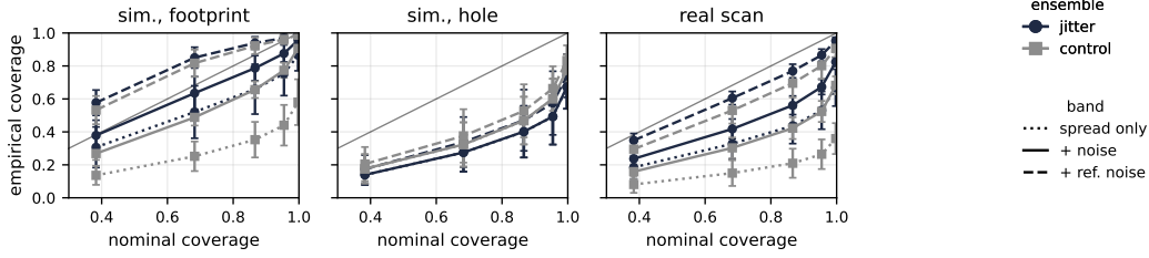
Figure 1: Coverage of |\text{mean} - \text{truth}| \leq z\sigma vs the Gaussian target, jitter (navy) and control (grey); dotted: spread only, solid: plus propagated noise, dashed: plus reference-map noise (sim upper bound; the correct band on the real scan). Bars: sd over lines and cases. Left: 32 simulated cases (footprint); middle: in a 14 \times 20 hole; right: the real scan.
