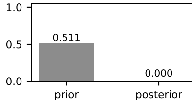
P(bilinear sampling)
