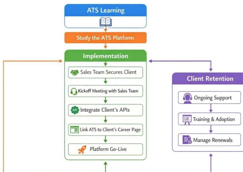
Fig 5.2 : Recruitment Workflow
