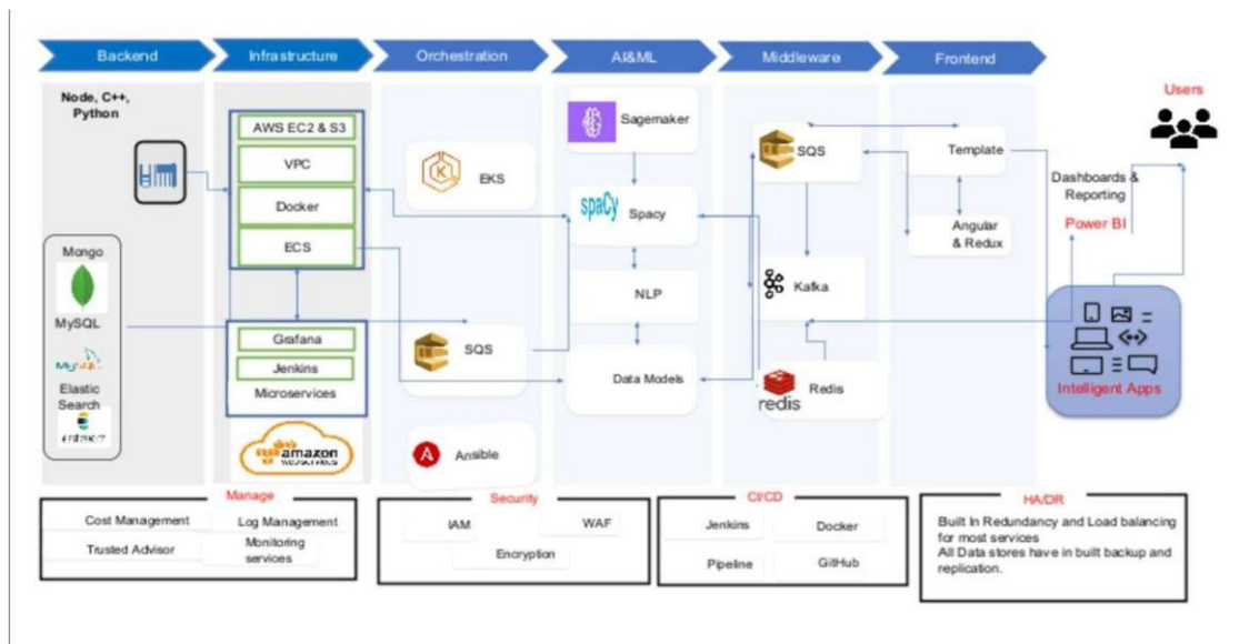
Fig 5.1 : System Architecture
