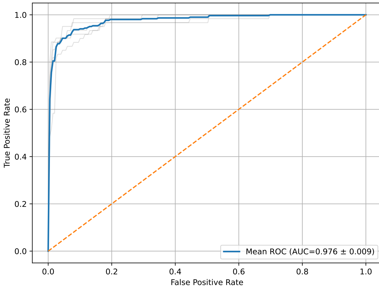
ROC - LGB
