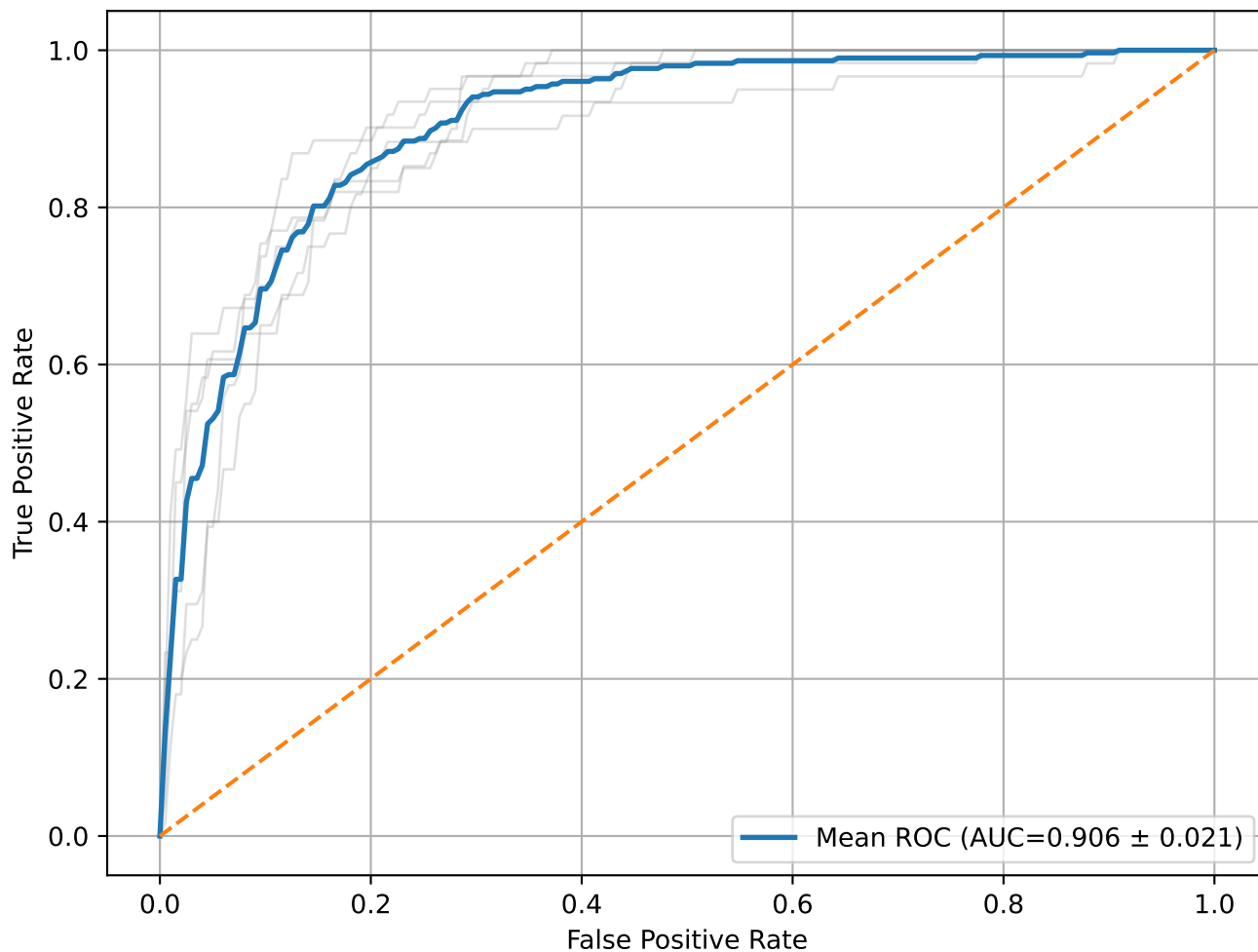
ROC - BAGGING
