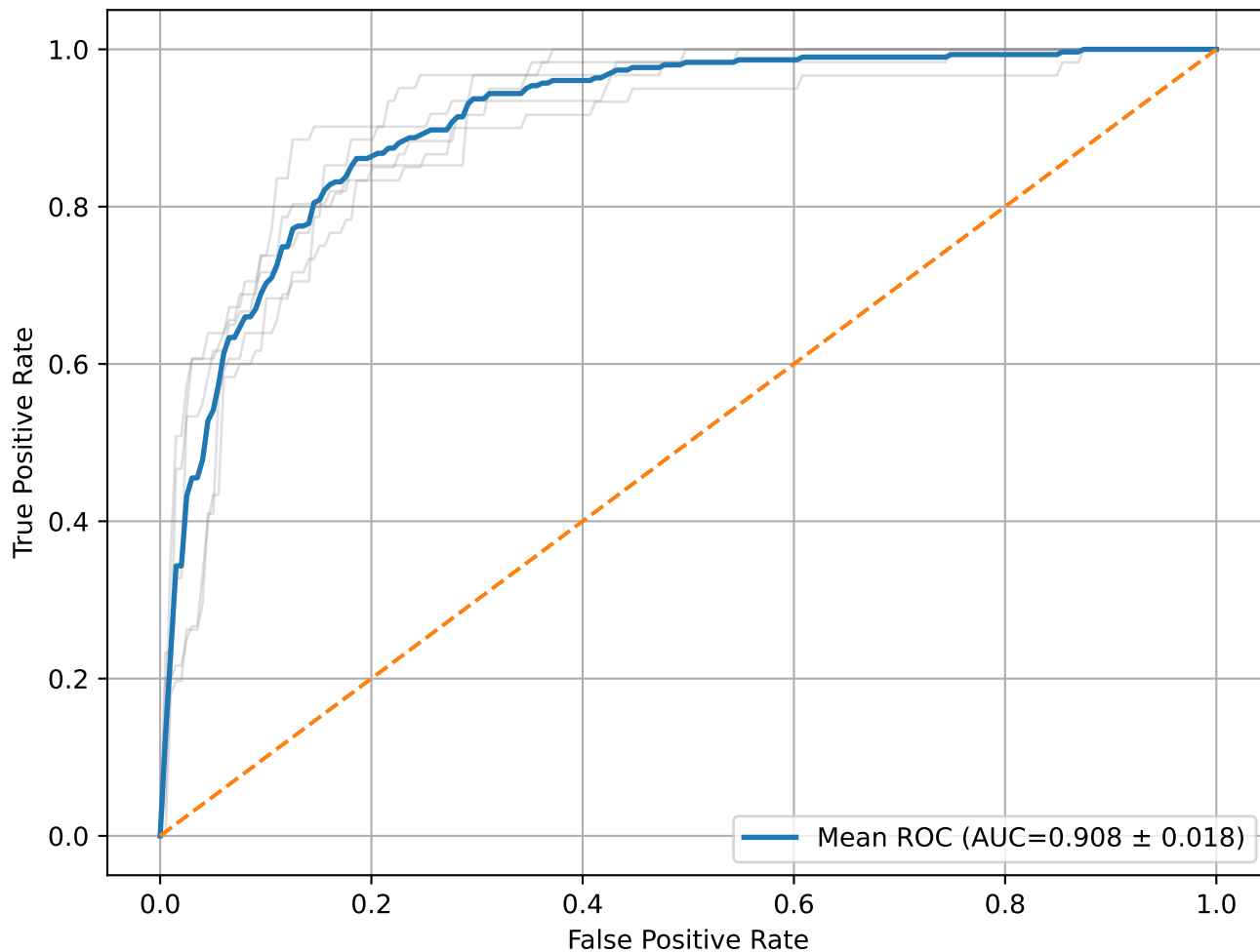
ROC - LOGISTIC
