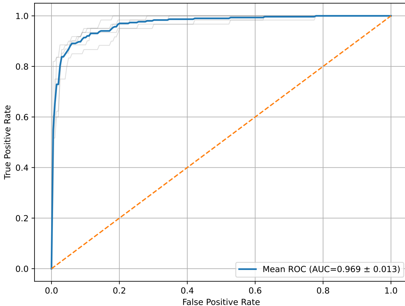
ROC - VOTING
