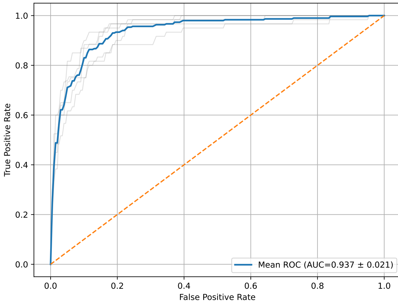
ROC - XGBOOST
