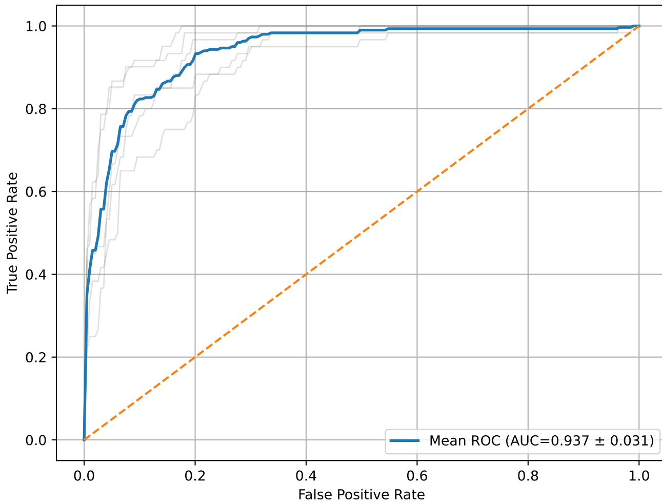
ROC - LIGHTGBM
