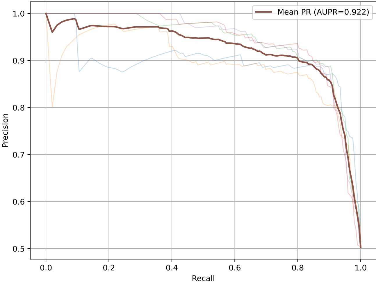
Precision-Recall - RF
